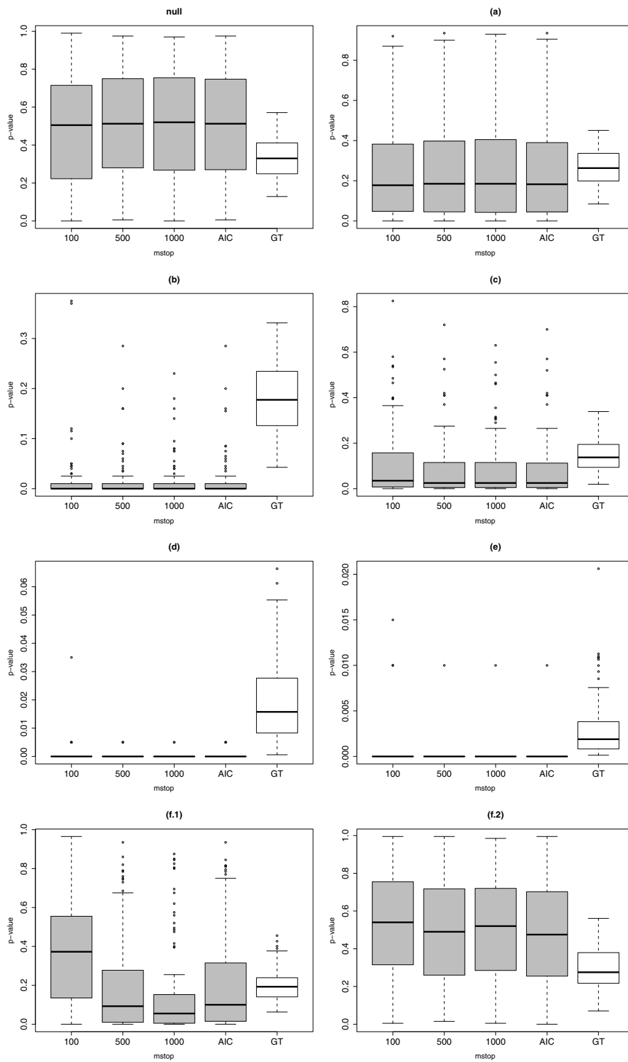
Figure 2 Boxplots of p-values. Boxplots of the p-values for the eight settings described in the Section 'Simulation design' using our new method with m_{stop} = 100, 500, 1000 and AIC-optimized m_{stop} (grey boxes) and using Goeman's global test (white boxes) for comparison.
