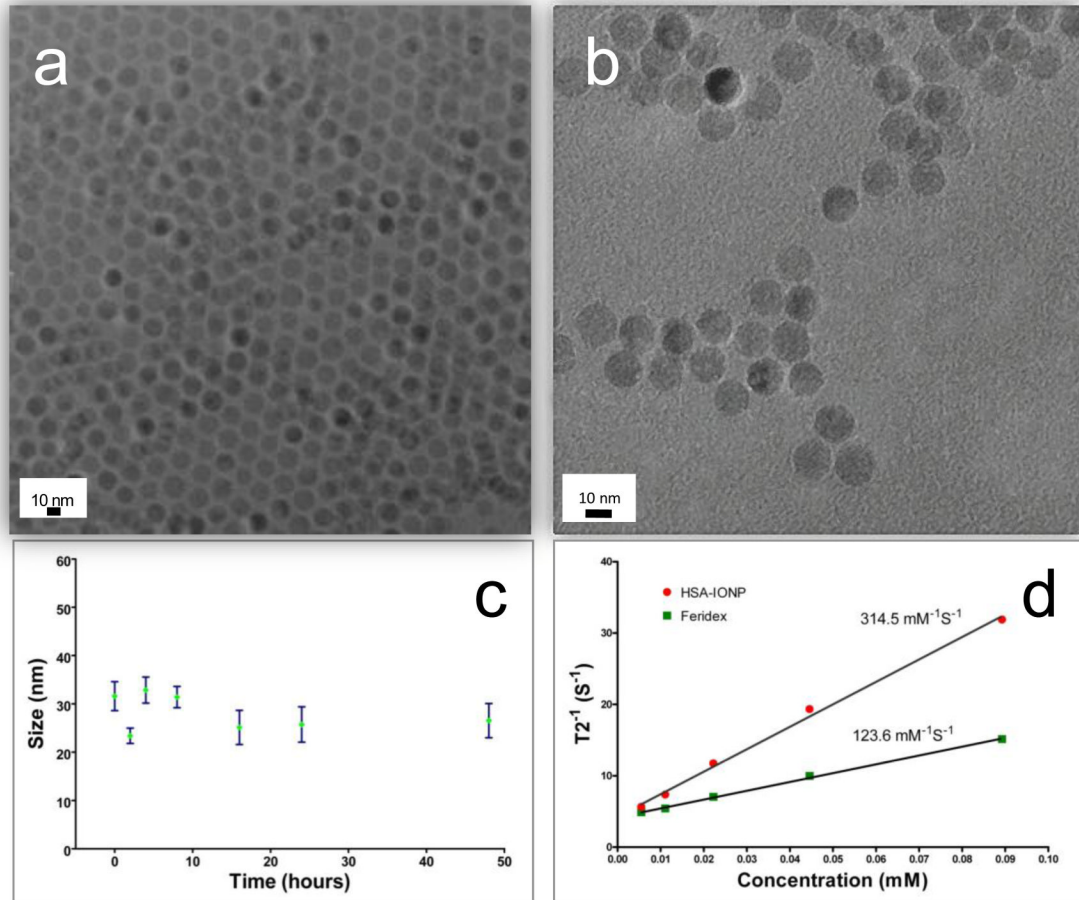
Fig. 2. (a) TEM of oleate coated IONPs in hexane. (b) TEM of the HSA-IONPs in water. (c) Hydrodynamic size change of the HSA-IONPs when incubating in PBS at 37°C for 48 hours, monitored by DLS. (d) r_2 relaxivity evaluations with HSA-IONPs and Feridex.
