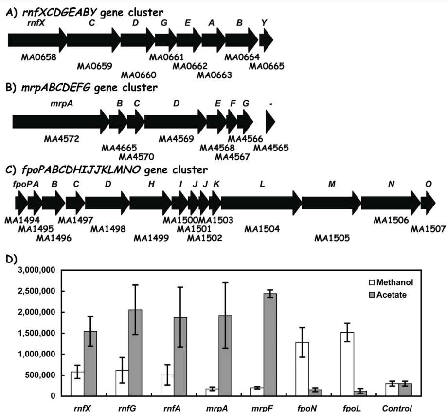
Figure 4 Differential expression of genes related to electron transport in M. acetivorans . The orientation and relative length of each gene is indicated by the open arrows. The Genbank identification number (MA number) is shown below each gene. Panels: A) The eight gene rnf cluster; B) the seven gene mrp cluster; C) the fourteen gene fpo cluster; and D), RT-PCR data for the indicated rnf , mrp , and fpo genes.
