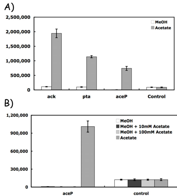
Figure 6 Differential expression of genes induced in presence of acetate. Panel A) The indicated genes include ack (acetate kinase), pta (phosphoacetyl transferase), and a gene designated aceP encoding a putative acetate uptake system. The RT-PCR data were determined as described in Materials. Panel B) Transcript abundance for aceP from cells grown in the presence or absence of the methanogenic substrate, methanol with the indicated amounts of acetate present.
