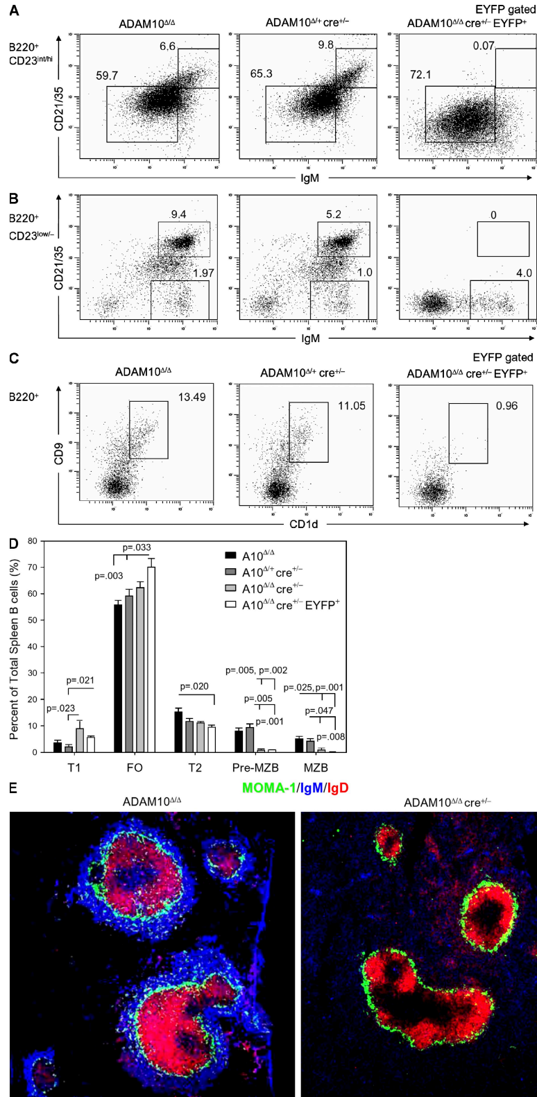
Figure 2. ADAM10 is essential for MZB lineage development. (A and B) Flow cytometric analysis of spleen B cells labeled for CD21/35 and IgM expression, gated on (A) B220 + CD23 int/hi and (B) B220 + CD23 low/- cells. (C) Analysis of PMZBs and MZBs labeled for CD1d and CD9 expression. Flow cytometric plots in A–C are representative of six experiments. (D) Levels of B cell subsets are expressed as the percentage of total spleen B cells ( n = 6 except for T2 cells [ n = 3 ]). Data are cumulative from six independent experiments for all subsets except for T2 cells, which are cumulative from three
