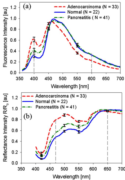
Fig. 1 (a) Mean fluorescence spectra obtained from human pancreatic normal (blue solid line), pancreatitis (green dot-dash line), and adenocarcinoma (red dashed line) tissues. The gray vertical dashed lines indicate the wavelengths at which F_{ratio}(=F_{400}/F_{600}) was calculated for each spectrum. (b) Mean reflectance spectra obtained from normal (blue solid line), pancreatitis (green dot-dash line), and adenocarcinoma (red dashed line) tissues. The gray dashed lines indicate the wavelengths at which R_{ratio}(=R_{470}/R_{650}) was calculated for each spectrum. N denotes the number of individual spectra. The standard error is shown at select wavelengths. (Color online only.)
