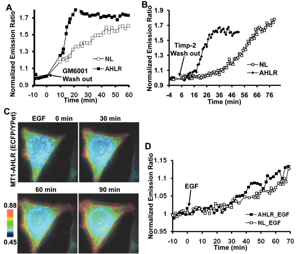
Figure 5. EGF induced a slow response of the optimized MT1-MMP biosensor. (A and B) The ECFP/YPet emission ratio changes of the NL ( \square ) and AHLR ( \blacksquare ) biosensors in response to (A) GM6001 or (B) Timp-2 washout. HeLa cells expressing MT1-MMP and biosensors were pre-incubated with (A) GM6001 ( 5\ \mu\text{M} ) or (B) Timp-2 ( 100\ \text{nM} ) for 12 hr, followed by the washout with HBSS or acid/neutralization solutions, respectively. (C) Representative ECFP/YPet emission ratio images of the optimized AHLR FRET biosensor upon EGF stimulation in HeLa cells expressing MT1-MMP. (D) The ECFP/YPet emission ratio time courses of the NL ( \square ) and AHLR ( \blacksquare ) biosensors before and after EGF stimulation in HeLa cells expressing MT1-MMP.
