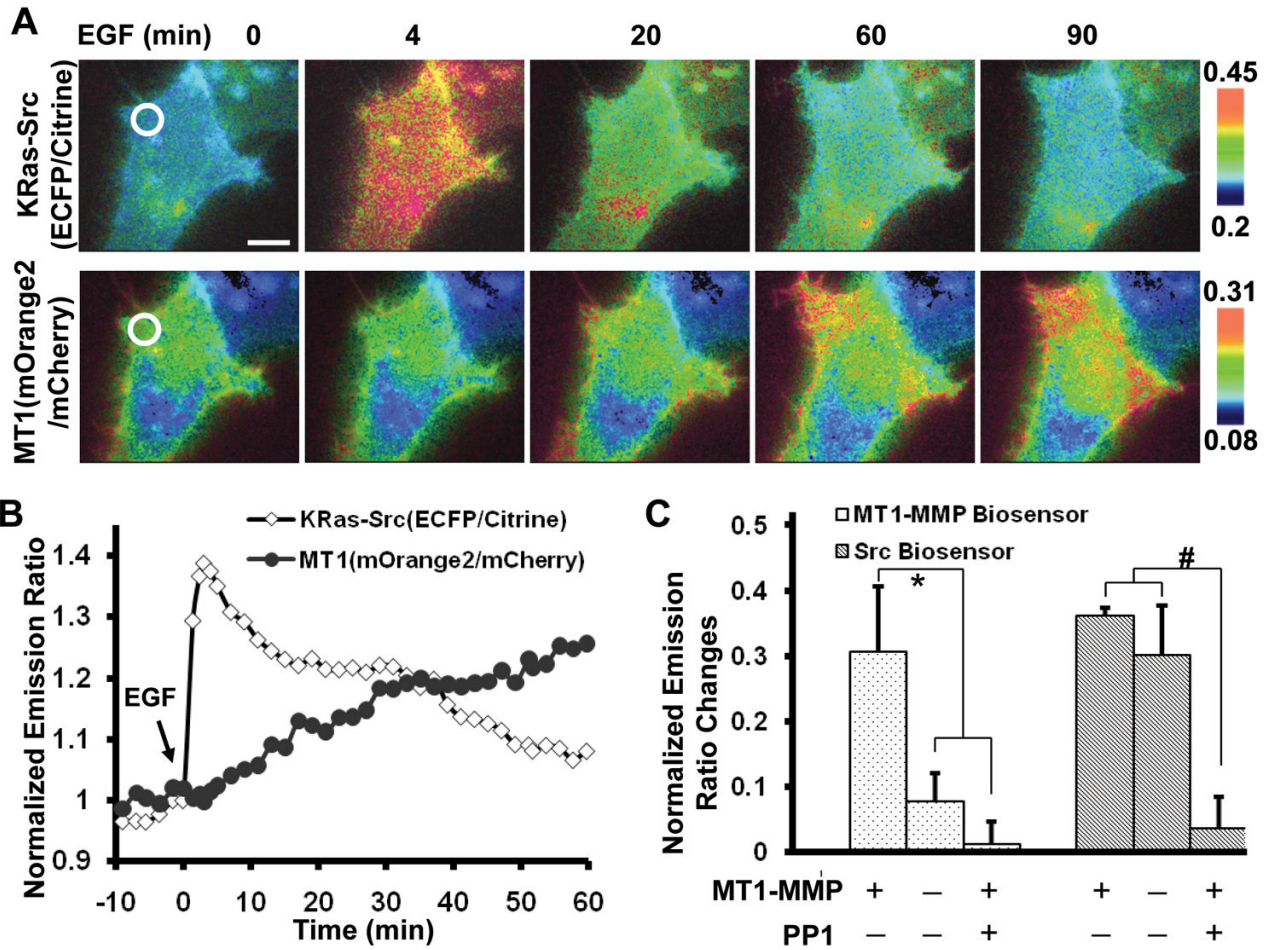
Figure 3. Concurrently visualizing the MT1-MMP and Src activities. (A) Emission ratio images of HeLa cells expressing Src (ECFP/Citrine, upper panels) and MT1-MMP (mOrange2/mCherry, lower panels) biosensors before and after EGF stimulation. (B) The normalized emission ratio time courses of the KRas-Src and MT1-MMP biosensors averaged on the chosen region of interest as indicated in (A). (C) Bar graphs show the emission ratio changes of the Src (ECFP/Citrine) and MT1-MMP (mOrange2/mCherry) biosensors in response to EGF. ‘MT1-MMP - ’ or ‘MT1-MMP + ’: HeLa cells co-transfected with a blank vector or MT1-MMP; ‘PP1 - ’ or ‘PP1 + ’: cells pretreated with DMSO or 10 \mu M PP1 for 1 hr. The * and # signs represent statistically significant difference between the indicated groups.
