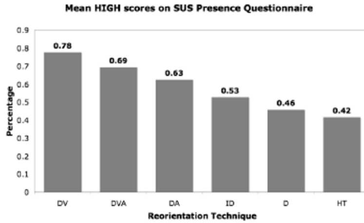
Fig. 18. Experiments 2 and 3—User rating - Mean percentage of HIGH scores on SUS Presence Questionnaire.
