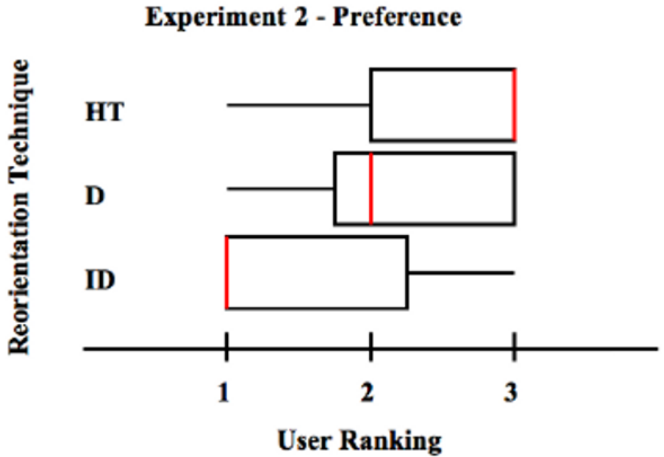
Fig. 13. Experiment 2—User rated preference scores from 1 (most preferred) to 3 (least preferred). Standard box-and-whisker plots with the median in red.
