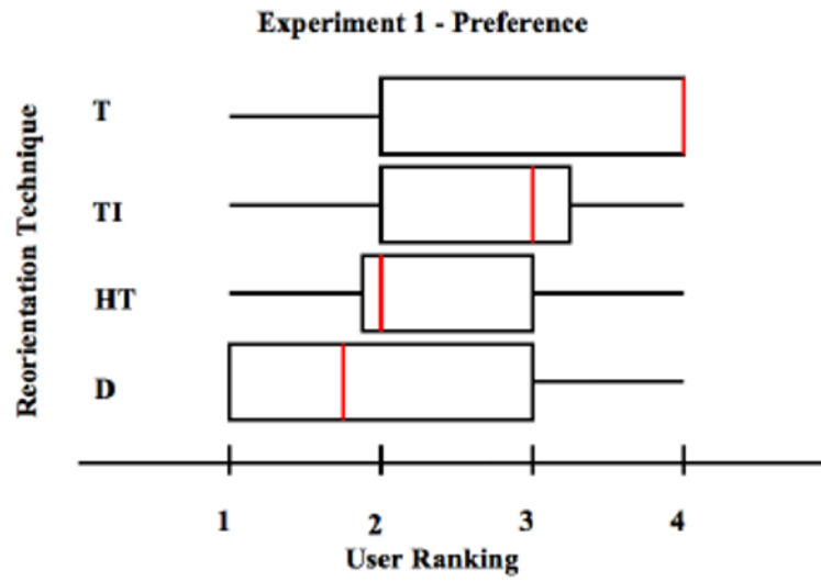
Fig. 5. Experiment 1–User rated preference scores from 1 (most preferred) to 4 (least preferred). Standard box-and-whisker plots with the median in red.
