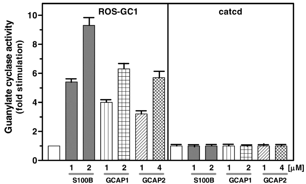
Figure 6. Specificity of the catcd V 837 -L 858 signal transduction site. The purified catcd fragment was assayed for guanylate cyclase activity in the presence of the indicated concentrations of S100B and 100 μM Ca 2+ or GCAP1 or GCAP2 in the presence of 10 nM Ca 2+ . Membranes of COS cell expressing ROS-GC1 were processed in parallel as the control. The experiment was done in triplicate and repeated two times with separate protein preparations. The results presented (mean ± SD) are from one experiment.
