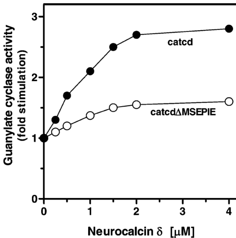
Figure 7. Effect of neurocalcin \delta on the guanylate cyclase activity of the catcd \Delta MSEPIE . The catcd \Delta MSEPIE mutant was assayed for guanylate cyclase activity in the presence of increasing concentrations of neurocalcin \delta and 100 \mu\text{M Ca}^{2+} . The catcd (control) was treated identically. The experiment was done in triplicate and repeated four times. The results presented are from one experiment. The error bar is within the size of the symbol.
