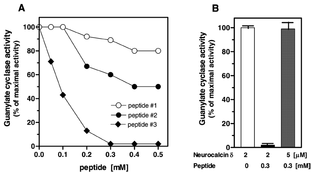
Figure 4. Peptide competition. (A) Inhibition of ROS-GC1 activity. Membranes of COS cells expressing ROS-GC1 were incubated with increasing concentrations of a peptide in the presence of 2 \mu M neurocalcin \delta and 100 \mu M \text{Ca}^{2+} . (B) Reversal of inhibition by an excess of neurocalcin \delta . Membranes of COS cells expressing ROS-GC1 were incubated with 2 \mu M neurocalcin \delta (open bars), 2 \mu M neurocalcin \delta and 0.3 mM peptide (closed bars), or 5 \mu M neurocalcin \delta and 0.3 mM peptide (checkered bars) and assayed for guanylate cyclase activity as in (A). Experiments were carried out in triplicate and repeated twice. The data shown are from a representative experiment.
