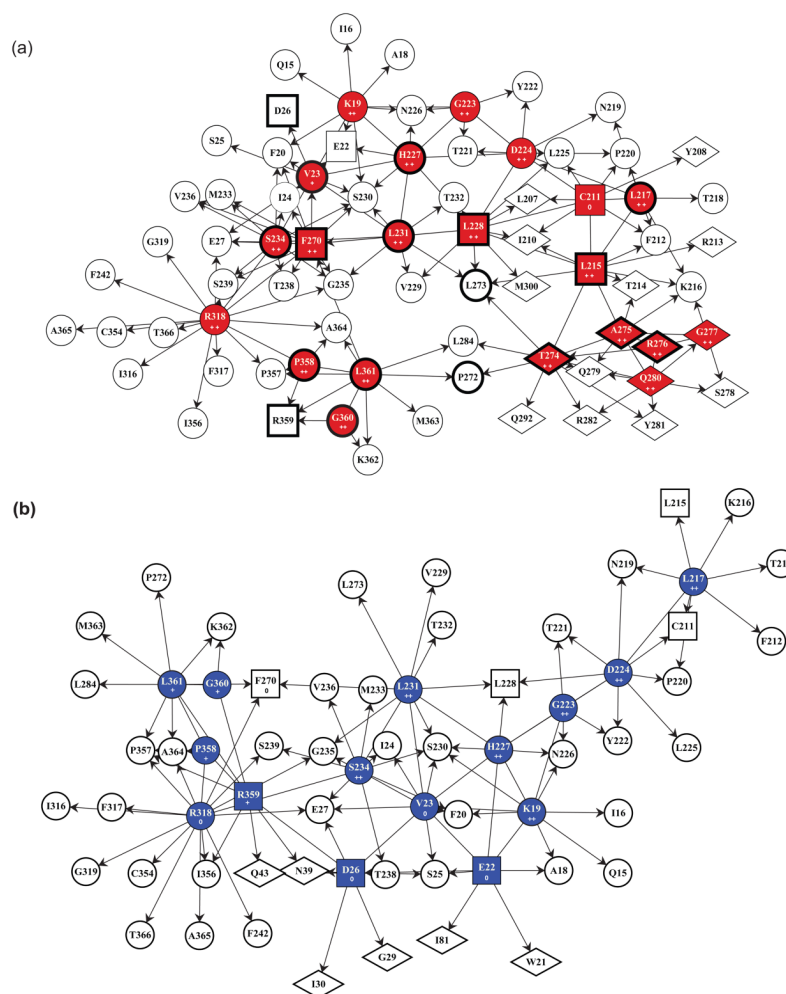
Figure 7. Contact maps of Taxol (a) and discodermolide (b) with chicken erythrocyte tubulin. In color (red for Taxol, and blue for discodermolide) are the residues in \beta -tubulin that make primary contacts with the corresponding drug. Clear shapes represent secondary contacts, those that interact with primary ones, but not the drug itself. Residues in squares are represented in both contact maps, but as primary contacts in one and secondary in the other. Residues in diamonds are unique to the corresponding drug. Those in circles are shared between the two drugs. Pluses and zeros are used to designate correspondence with changes in HDX of peptides containing the indicated amino acid residues: ++ indicates a large significant decrease in labeling ( \Delta\text{HDX} > 0.5 ), + indicates a small but significant decrease in labeling ( \Delta\text{HDX} > 0 ), and 0 indicates no effect on labeling ( \Delta\text{HDX} = 0 ). In (a), residues that have been previously shown to interact with Taxol are boxed in bold. 8
