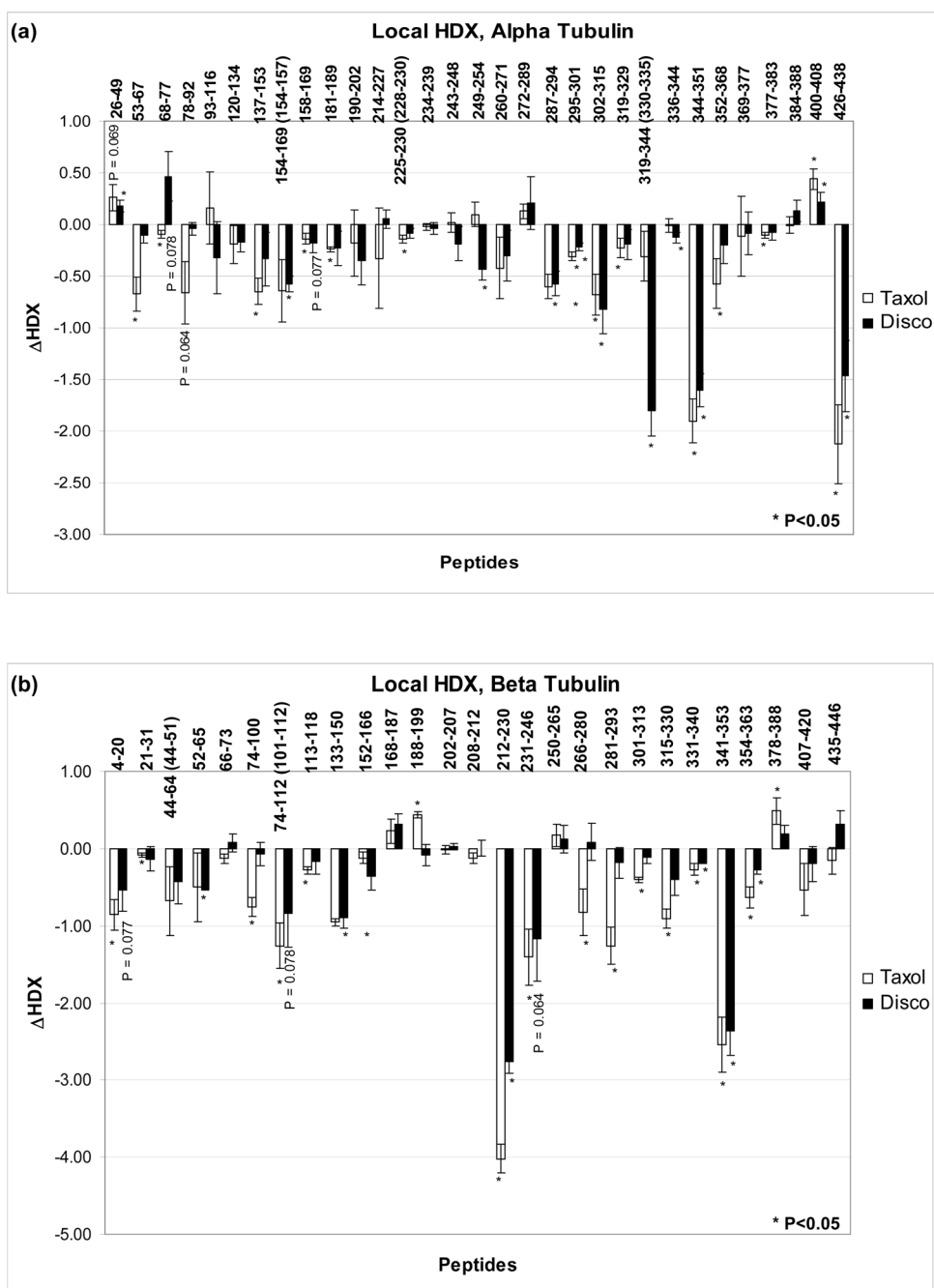
Figure 3. Drug-induced alterations in deuteration referenced against GMPCPP-stabilized microtubules for (a) \alpha -tubulin and (b) \beta -tubulin. Data indicate the mean \pm standard deviation of three separate experiments. Differences in deuteration ( \Delta HDX) are expressed as mass units. For overlapping peptides, unique residues are indicated in parentheses. All peptides with significant alterations in deuterium incorporation ( P < 0.05 ) are marked with an asterisk. Some relevant peptides with average \Delta HDX values just outside the significance level are labeled with their respective P values.
