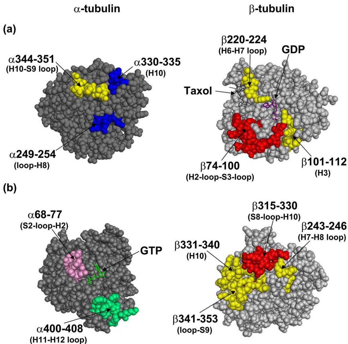
Figure 6. Mapping the local HDX alterations on the (a) inter- and (b) intradimer interfaces of the tubulin dimer (1JFF). The peptides are colored according to the code in Fig. 4. Briefly, peptic peptides labeled in blue are more protected by discodermolide; in red are more protected by Taxol; in yellow are protected similarly by both drugs; in green are deprotected similarly by both drugs; and in pink are deprotected by discodermolide, but unaffected by Taxol. Secondary structure designations are based on Löwe et al. 8
