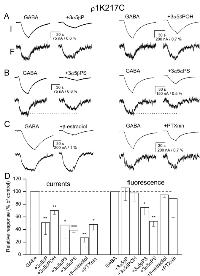
Fig. 2. Current and fluorescence responses from the \rho 1 receptor labeled with A5m at the K217C site. Current and fluorescence responses from receptors activated by 1 \mu\text{M} GABA in the absence and presence of 20 \mu\text{M} 3\alpha 5\beta\text{P} or 3\alpha 5\beta\text{POH} (A), 3\alpha 5\beta\text{PS} or 3\alpha 5\alpha\text{PS} (B), or \beta -estradiol or 10 \mu\text{M} picrotoxinin (PTXnin) (C). The top traces show currents (I), and the bottom traces show the concomitant changes in fluorescence (F). The modulators are sorted according to their proposed classification into groups. All drugs inhibit the electrophysiological response, but only 3\alpha 5\beta\text{PS} and 3\alpha 5\alpha\text{PS} reduce the change in fluorescence (shown with dotted lines). D, the summary of effects on electrophysiology and fluorescence responses. *, p < 0.05 ; **, p < 0.01 ; ***, p < 0.001 .
