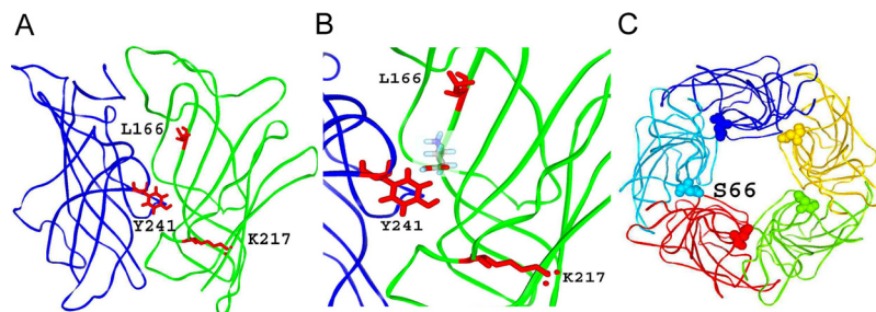
Fig. 1. Structures of the GABA receptor. A, structural model of the extracellular domain of the human \rho 1 GABA receptor. The model was constructed by homology with the acetylcholine-binding protein. The model shows two neighboring subunits (blue and green) containing a single transmitter binding pocket. B, a higher-resolution image of the transmitter binding pocket. Three of the four residues used for labeling with A5m are shown with molecular structures (Tyr241 of the “+” side of the interface, and Lys217 and Leu166 of the “-” side of the interface are shown in red). A GABA molecule is placed in the putative transmitter binding pocket. C, a top view of the receptor showing the Ser66 residue located near the subunit-subunit interface in each of the five subunits of the GABA receptor.
