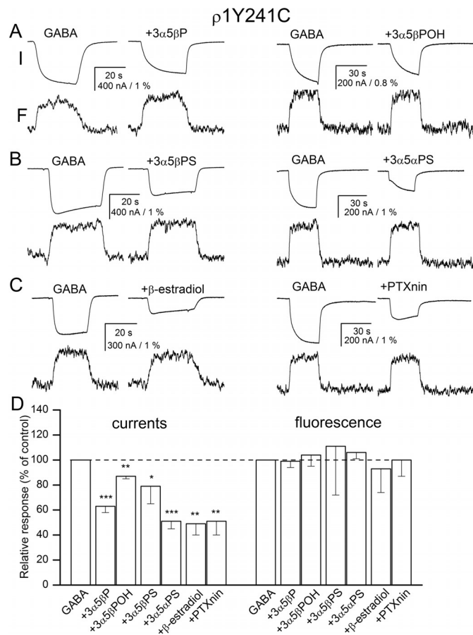
Fig. 5. Current and fluorescence responses from the \rho 1 receptor labeled with A5m at the Y241C site. Current and fluorescence responses from receptors activated by 5 \mu M GABA in the absence and presence of 20 \mu M 3\alpha 5\beta P or 3\alpha 5\beta POH (A), 3\alpha 5\beta PS or 3\alpha 5\alpha PS (B), or \beta -estradiol or 10 \mu M picrotoxinin (PTXnin) (C). The top traces show currents (I) and the bottom traces show the concomitant changes in fluorescence (F). The modulators are sorted according to their proposed classification into groups. All drugs inhibit the electrophysiological response. None of the drugs affects the change in fluorescence. D, the summary of effects on electrophysiology and fluorescence responses. *, p < 0.05 ; **, p < 0.01 ; ***, p < 0.001 .
