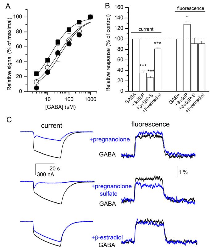
Fig. 6. Current and fluorescence responses from the \rho 1T298F receptor labeled with A5m at the L166C site. A, GABA concentration-effect relationships for currents (○, unlabeled \rho 1L166C + T298F mutant receptors; ●, receptors labeled with A5m) and fluorescence changes (■, receptors labeled with A5m). The curves were fitted to the Hill equation. The best-fit parameters for currents from unlabeled receptors are EC_{50} = 30 \pm 4 \mu M, n_H = 0.8 \pm 0.1 . The best-fit parameters for currents from receptors labeled with A5m are EC_{50} = 40 \pm 9 \mu M, n_H = 0.8 \pm 0.1 . The best-fit parameters for fluorescence from receptors labeled with A5m are EC_{50} = 14 \pm 1 \mu M, n_H = 0.8 \pm 0.1 . B, summary of steroid effects on electrophysiology and fluorescence responses. 3\alpha 5\beta P , pregnanolone; 3\alpha 5\beta PS , pregnanolone sulfate. *, p < 0.05 ; **, p < 0.01 ; ***, p < 0.001 . C, sample current and fluorescence traces from the \rho 1L166C + T298F receptors. The traces show responses to 30 \mu M GABA in the absence and presence of 20 \mu M pregnanolone (top), pregnanolone sulfate (middle), or \beta -estradiol (bottom). The data indicate that the T298F mutation reduces the ability of \beta -estradiol to inhibit the current and fluorescence responses (compare with Fig. 3C).
