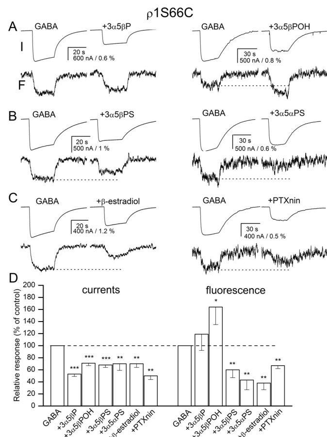
Fig. 4. Current and fluorescence responses from the \rho 1 receptor labeled with A5m at the S66C site. Current and fluorescence responses from receptors activated by 5 \mu\text{M} GABA in the absence and presence of 20 \mu\text{M} 3\alpha 5\beta\text{P} or 3\alpha 5\beta\text{POH} (A), 3\alpha 5\beta\text{PS} or 3\alpha 5\alpha\text{PS} (B), or \beta -estradiol or 10 \mu\text{M} picrotoxinin (PTXnin) (C). The top traces show currents ( I ), and the bottom traces show the concomitant changes in fluorescence ( F ). The modulators are sorted according to their proposed classification into groups. All drugs inhibit the electrophysiological response. The application of 3\alpha 5\beta\text{POH} enhances whereas the application of 3\alpha 5\beta\text{PS} , 3\alpha 5\alpha\text{PS} , \beta -estradiol or PTXnin reduce the change in fluorescence (shown with dotted lines). D, the summary of effects on electrophysiology and fluorescence responses. *, p < 0.05 ; **, p < 0.01 ; ***, p < 0.001 .
