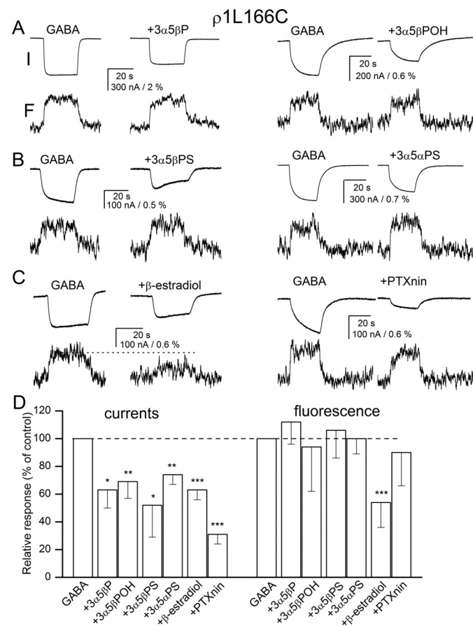
Fig. 3. Current and fluorescence responses from the \rho 1 receptor labeled with A5m at the L166C site. Current and fluorescence responses from receptors activated by 60 \mu\text{M} GABA in the absence and presence of 20 \mu\text{M} 3\alpha 5\beta\text{P} or 3\alpha 5\beta\text{POH} (A), 3\alpha 5\beta\text{PS} or 3\alpha 5\alpha\text{PS} (B), or \beta -estradiol or 10 \mu\text{M} picrotoxinin (PTXnin) (C). The top traces show currents (I), and the bottom traces show the concomitant changes in fluorescence (F). The modulators are sorted according to their proposed classification into groups. All drugs inhibit the electrophysiological response, but only \beta -estradiol reduces the change in fluorescence (shown with dotted line). D, the summary of effects on electrophysiology and fluorescence responses. *, p < 0.05 ; **, p < 0.01 ; ***, p < 0.001 .
