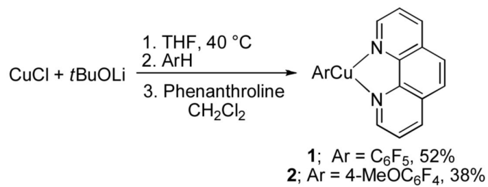
Scheme 16. Mechanistic Considerations
