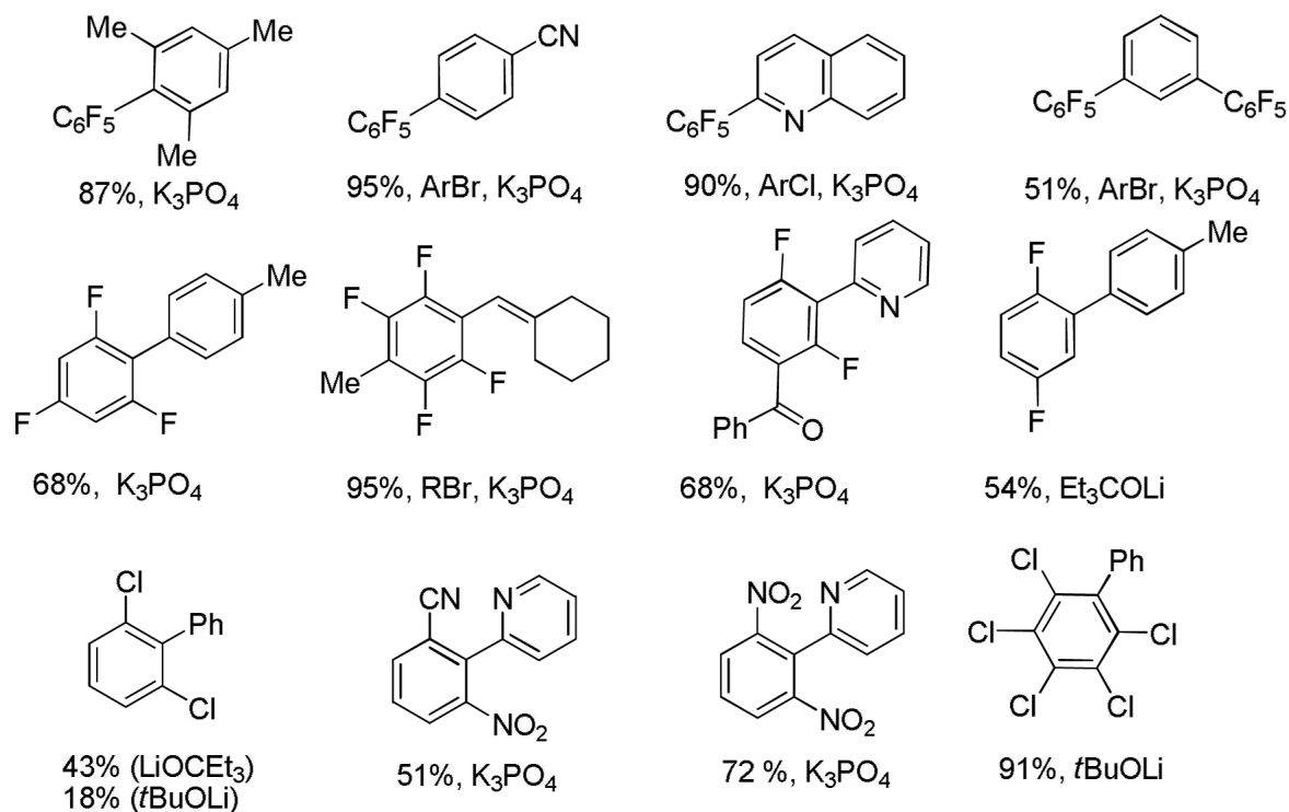
Scheme 15. Electron-Deficient Benzene Arylation
