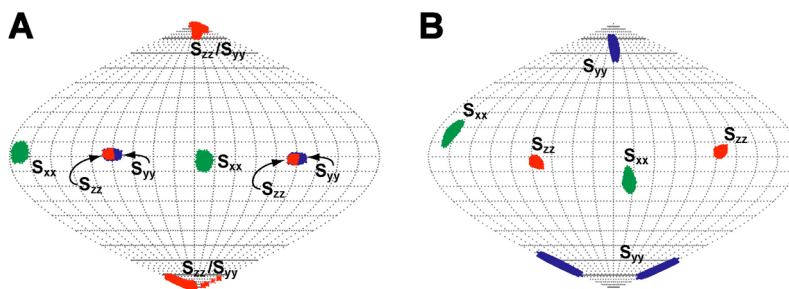
Figure 6. Sauson-Flaumsteed projection maps illustrating the orientations of the principal components of the molecular alignment tensor derived from alignment by (A) 10 mg/mL Pf1 and (B) MSA-induced alignment using the normalized average RDC values measured at 800 and 900 MHz, ^1D_{HN}(800, 900) . Areas of green, blue and red correspond to the orientations of the principal components of the order tensor S_{xx} , S_{yy} , and S_{zz} , respectively.
