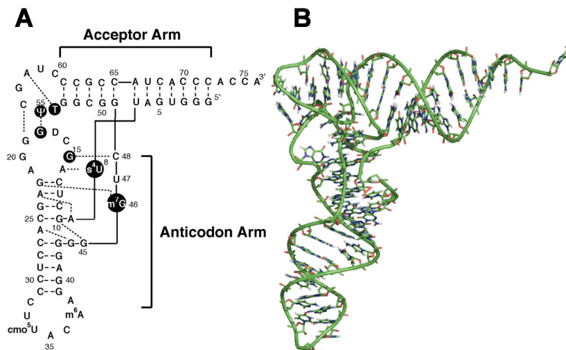
Figure 1. (A) Sequence and secondary structure and (B) tertiary structure model of native E. coli tRNA Val (Vermeulen, et al. 2005). (A) Long dashes represent canonical Watson-Crick base pairs and the short dashed lines represent non-canonical or tertiary interactions. Imino groups of the residues in black circles are involved in tertiary interactions, and their ^1D_{HN} values were omitted from SVD analysis. The two helical domains are labeled as the acceptor arm and the anticodon arm.
