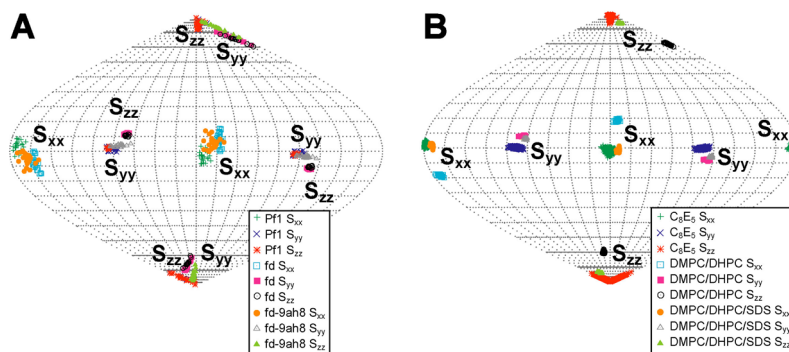
Figure 4. Sauson-Flaumsted projection maps illustrating the orientations of the principal components of the molecular alignment tensor for native E. coli tRNA Val derived from alignment by (A) various filamentous bacteriophage and (B) bilayer or bicelle alignment media. The positions of the principal components S_{xx} , S_{yy} and S_{zz} of the alignment are indicated on each map. The legend in the lower right of each map shows the symbols for the principal components for the various alignment media. Due to the high rhombicity for several of the alignment tensors, the orientations of S_{zz} and S_{yy} are exchanged. Sauson-Flaumsted projection maps were generated from the SVD output using the program REDCAT (Valafar and Prestegard 2004). 50 solutions are plotted for each alignment tensor.
