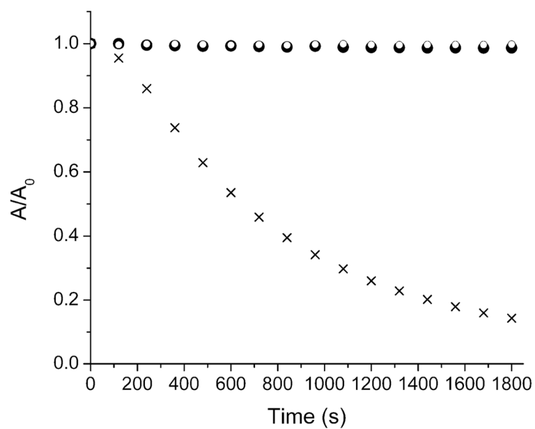
FIGURE 9. Change in absorption upon addition of 2-mercaptoethanol (50 mM) to 4 (●), 5 (○), and 1a (X) in CHCl 3 (10 μM) at 25 °C.
