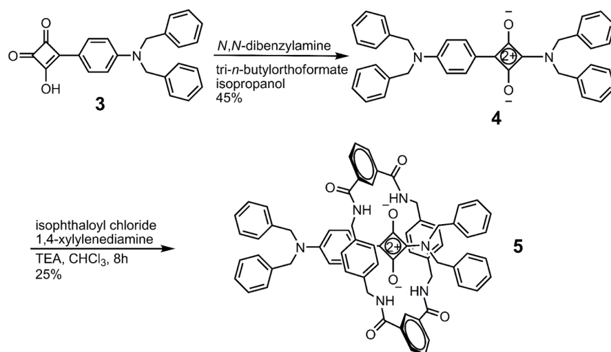
SCHEME 1. Synthesis of Truncated Rotaxane 5
