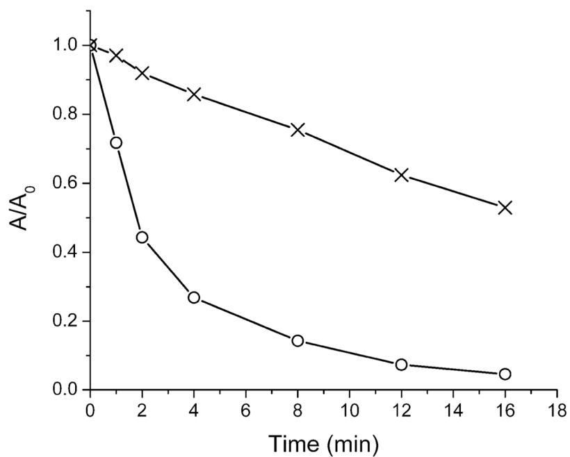
FIGURE 8. Change in absorption of 4 (○) and 5 (×) in \text{CHCl}_3 (10 \mu\text{M} ) upon exposure to an unfiltered xenon arc lamp (150 W) at 25 °C.
