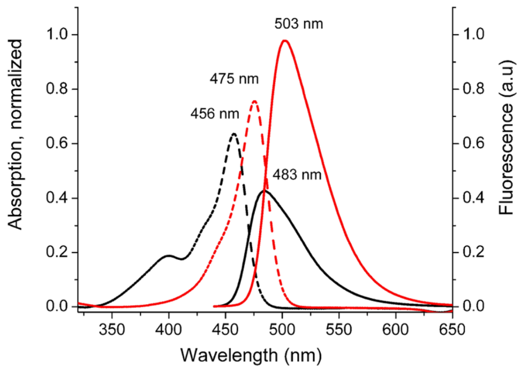
FIGURE 7. Absorption spectra of 4 (—, black) and 5 (---, red) and fluorescence emission spectra of 4 (—, black) and 5 (---, red) in \text{CHCl}_3 ( 5 \mu\text{M} ).
