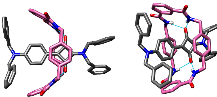
FIGURE 6. X-ray crystal structure of truncated squaraine rotaxane 5 .
