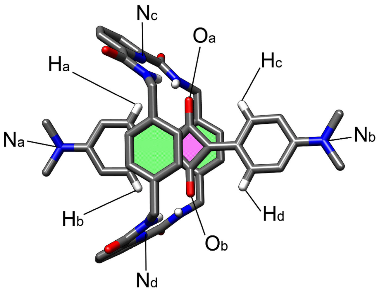
FIGURE 3. Atom labels for squaraine rotaxanes.
