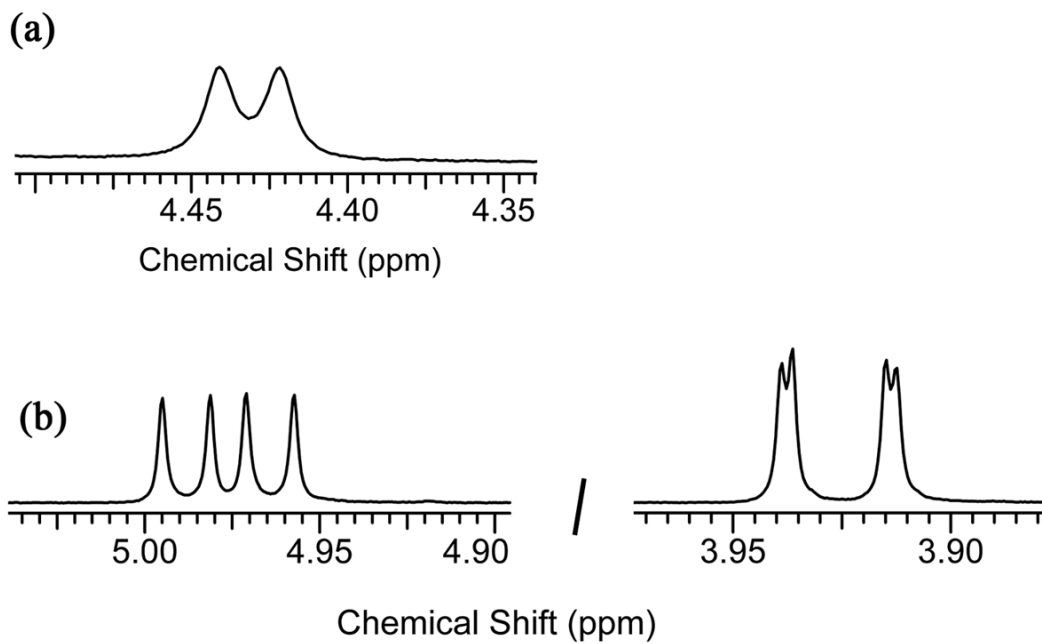
FIGURE 4. Partial ^1\text{H} NMR spectra at 22 °C in \text{CDCl}_3 showing the macrocycle methylene signals for squaraine rotaxanes; (a) 2d with J = 5.8 Hz in a 300 MHz spectrum; (b) 5 with J_1 = 8.2 Hz, J_2 = 14.4 Hz (left) and J_1 = 1.5 Hz, J_2 = 14.4 Hz (right) in a 600 MHz spectrum.
