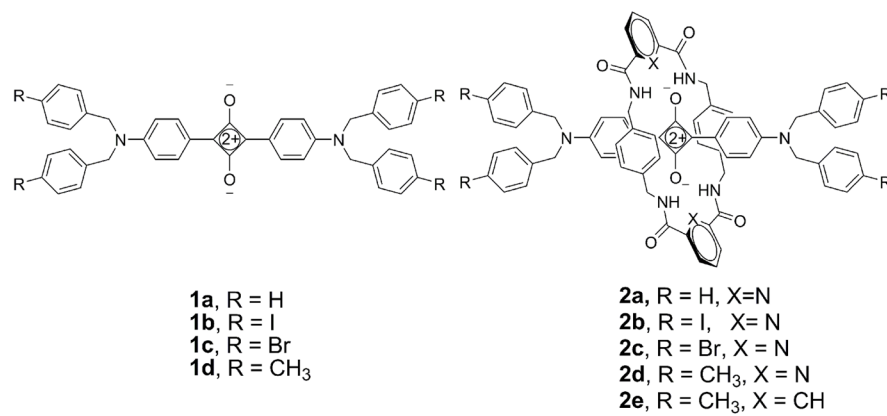
FIGURE 1. Squaraine dyes and squaraine rotaxanes.
