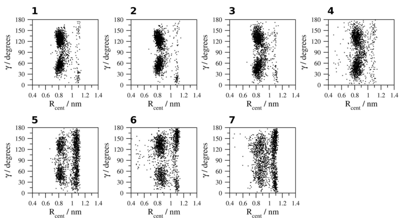
Figure 11. Geometric analysis of the relative orientation of the aromatic rings of Tyr1 and Tyr2. 1 , H 2 O (278 K); 2 , H 2 O (300 K); 3 , H 2 O (333 K); 4 , H 2 O (363 K); 5 , TFE; 6 , MeOH and 7 , DMSO.
