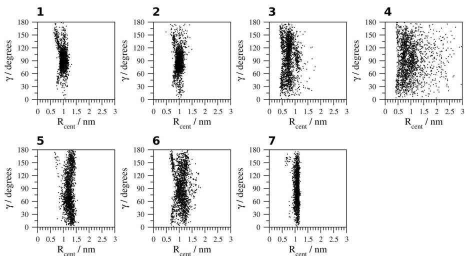
Figure 9. Geometric analysis of the relative orientation of the aromatic rings of Tyr1 and Trp9. 1 , H 2 O (278 K); 2 , H 2 O (300 K); 3 , H 2 O (333 K); 4 , H 2 O (363 K); 5 , TFE; 6 , MeOH and 7 , DMSO.
