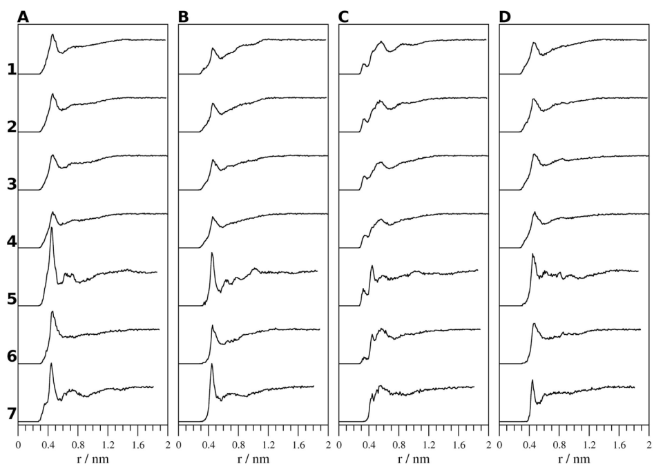
Figure 6. Radial distribution functions between the center of mass of the aromatic rings of A , Tyr1; B , Tyr2; C , Trp9; and D , Tyr10 and the oxygen atoms in the solvent from the simulations of 1 , H 2 O (278 K); 2 , H 2 O (300 K); 3 , H 2 O (333 K); 4 , H 2 O (363 K); 5 , TFE; 6 , MeOH; and 7 , DMSO.
