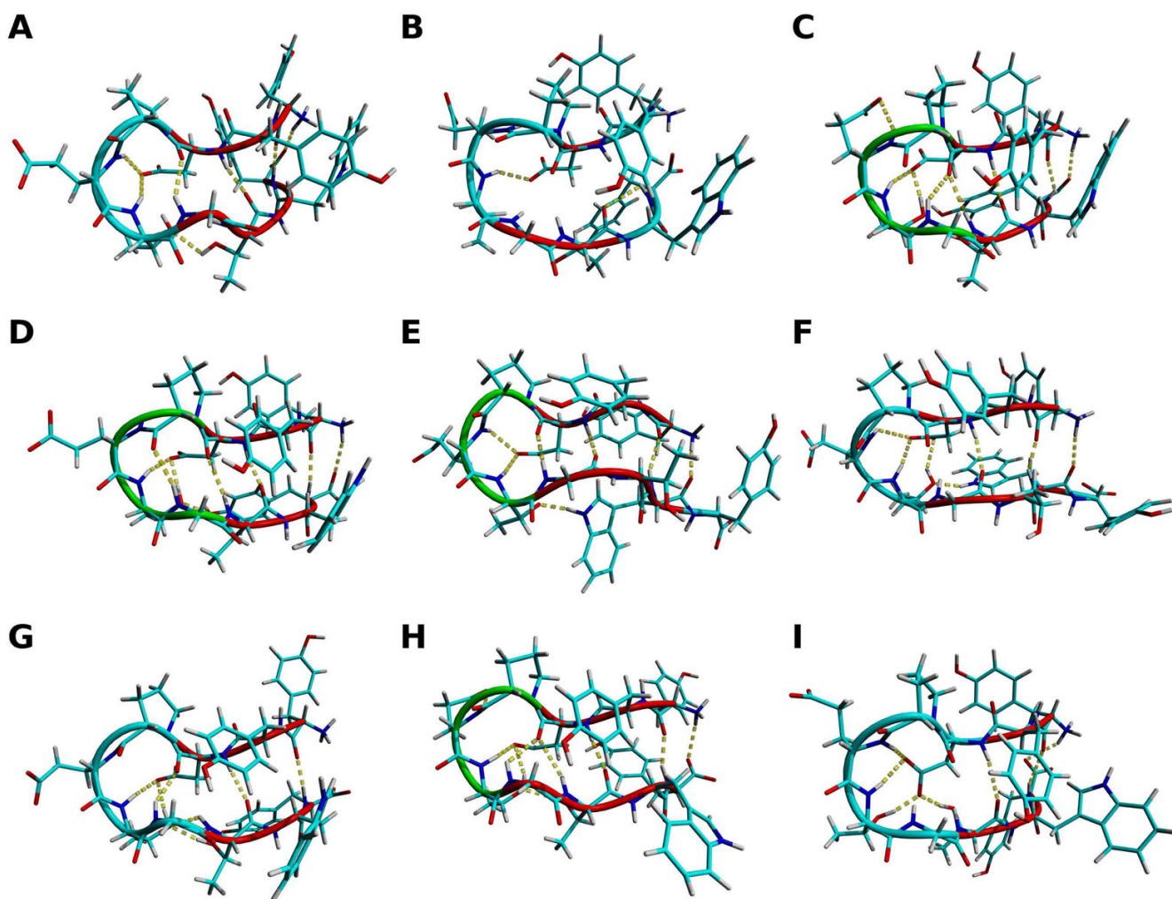
Figure 3. The backbone and side chains of CLN025. A , X-ray structure 27 ; B , the first NMR structure 27 and the middle structures of the most populated clusters of the trajectories of the MD simulations of CLN025 in C , H 2 O (278 K); D , H 2 O (300 K); E , H 2 O (333 K); F , H 2 O (363 K); G , TFE; H , MeOH and I , DMSO. Random meander is cyan, \beta -sheet is red, turn is green and the H-bonds are yellow dotted lines.
