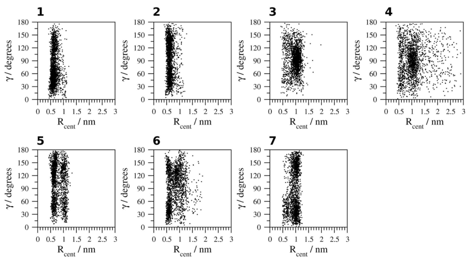
Figure 8. Geometric analysis of the relative orientation of the aromatic rings of Tyr1 and Tyr10. 1 , H 2 O (278 K); 2 , H 2 O (300 K); 3 , H 2 O (333 K); 4 , H 2 O (363 K); 5 , TFE; 6 , MeOH and 7 , DMSO.
