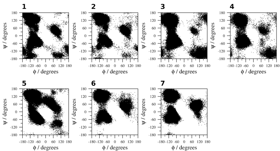
Figure 4. \phi and \psi dihedral angles of the residues of CLN025 along the trajectories of the MD simulations. 1 , \text{H}_2\text{O} (278 K); 2 , \text{H}_2\text{O} (300 K); 3 , \text{H}_2\text{O} (333 K); 4 , \text{H}_2\text{O} (363 K); 5 , TFE; 6 , MeOH and 7 , DMSO.
