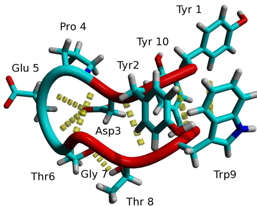
Figure 2. The backbone and side chains of the NMR structure of CLN025 27 . Random meander is cyan, \beta -sheet is red, turn is green and the H-bonds are yellow dotted lines.
