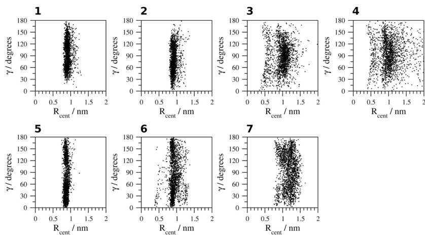
Figure 10. Geometric analysis of the relative orientation of the aromatic rings of Tyr2 and Tyr10. 1 , H 2 O (278 K); 2 , H 2 O (300 K); 3 , H 2 O (333 K); 4 , H 2 O (363 K); 5 , TFE; 6 , MeOH and 7 , DMSO.
