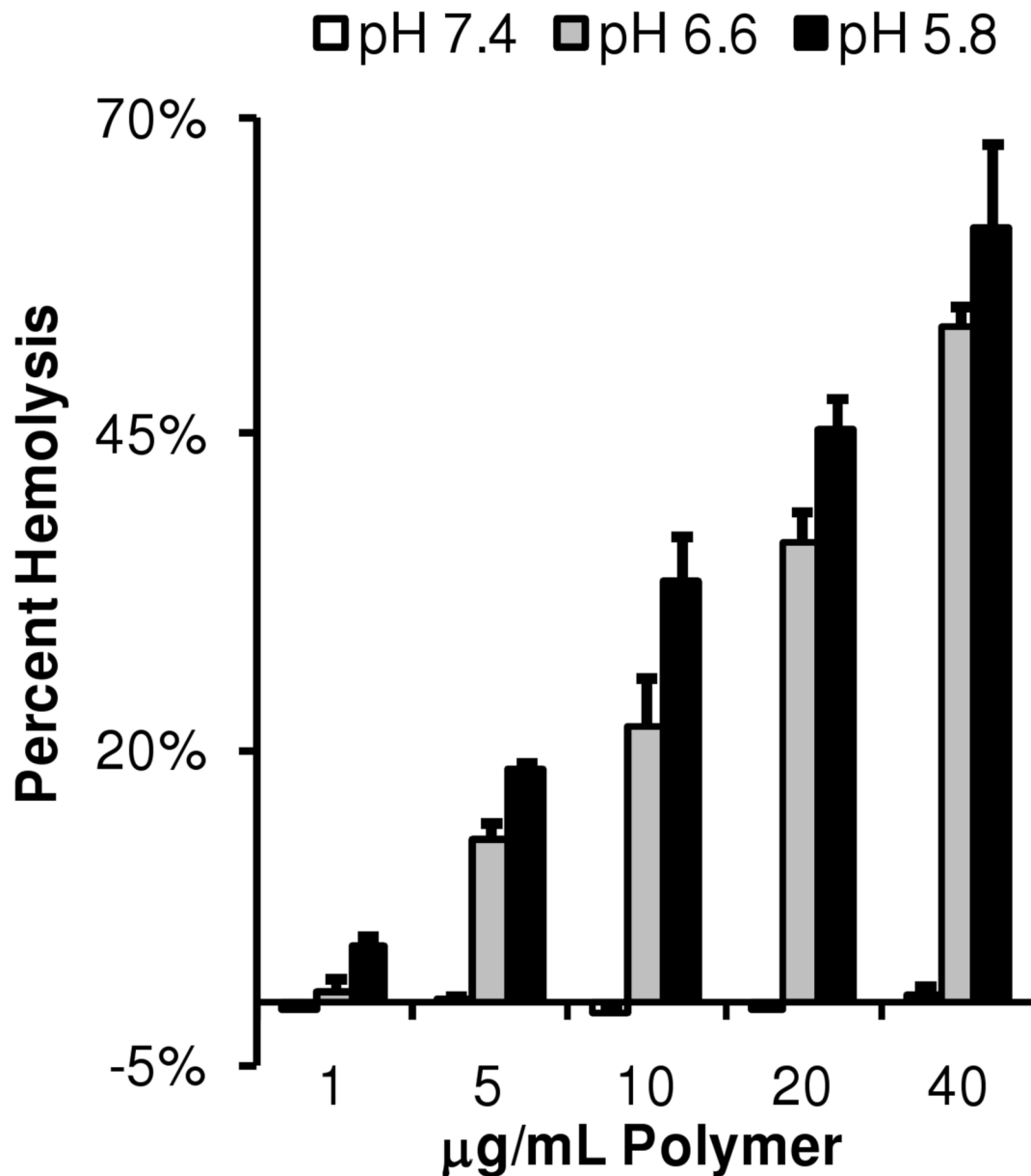
Figure 2. pH-dependent membrane disruption by poly[HPMA]-b-[(PAA)(BMA)(DMAEMA)] Polymer hemolysis was quantified at concentrations ranging from 1-40 µg/mL relative to 1% v/v Triton X-100. This experiment was completed 2 times in triplicate, yielding similar results. The data shown represent a single experiment conducted in triplicate \pm standard deviation.
