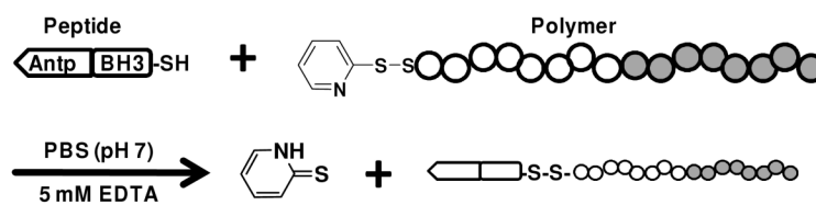
Scheme 2. Polymer-peptide conjugation via thiol-disulfide exchange reaction
