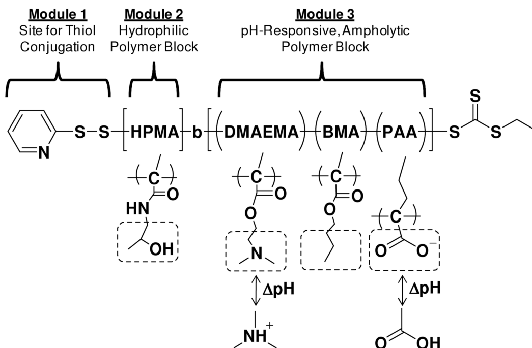
Figure 1. Poly[HPMA]-b-[(PAA)(BMA)(DMAEMA)] polymer design
