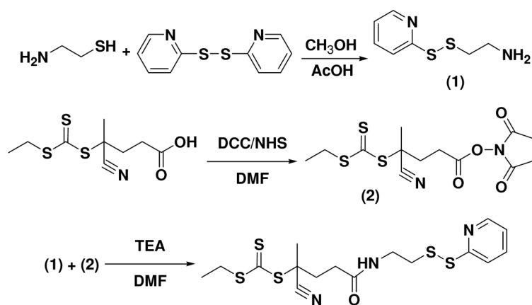
Scheme 1. Synthesis of Pyridyl Disulfide CTA
