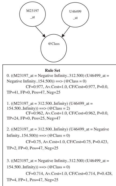
Fig. 1. A BN structure learned by BRL on the acute lymphoblastic leukemia (ALL) versus acute myeloid leukemia (AML) dataset (Golub et al. , 1999) and its equivalent set of rules. @Class refers to the target variable that can take on values of either 0 (ALL) or 2 (AML) in this example. Each rule is associated with statistics from the training data (see note 1).
