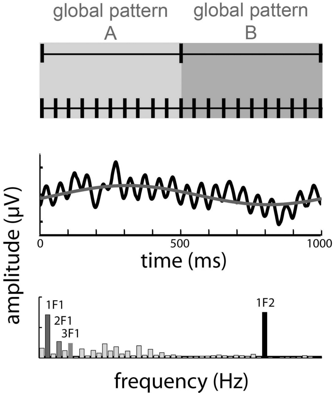
Figure 3. Response component analysis. [TOP] The global structure of the Glass pattern stimuli alternated at a rate of 1 Hz (i.e. changed every 500 ms), while their local elements were updated at a rate of 20 Hz (i.e., changed every 50 ms). [MIDDLE] The event-related waveforms reflect the structure of the stimulus presentation, which exhibits high frequency modulation (black) riding on top of a low frequency component (red). [BOTTOM] Decomposition of the waveform into its spectral components isolates the responses to the global (1–3 Hz) and local (20 Hz) structure of the Glass pattern stimuli in specific frequency bins that are tightly tied to the local and global update rates. Statistical analyses were performed on the spectral components of the responses.
