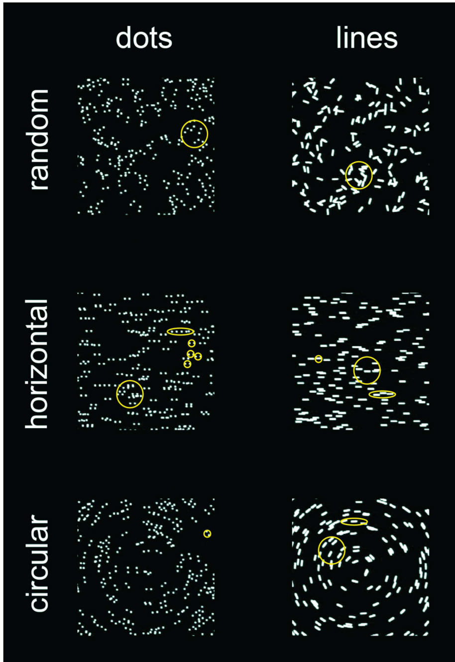
Figure 1. Examples (to scale) of Glass patterns and corresponding line patterns. Dot pairs and lines were [TOP] randomly oriented, [MIDDLE] aligned horizontally and [BOTTOM] aligned co-circularly. In the first experiment, the patterns alternated between horizontal and random global organizations. In subsequent experiments, the patterns alternated between co-circular and horizontal global organizations. Our model (yellow outlines) proposes that infants have isotropic integration fields (large circles), but lack collinear specific integration fields (ovals) that allow extraction of orientation signals in Glass patterns. Small circles represent receptive fields. Note that dots, but not lines, within isotropic integration fields appear to have random structure.
