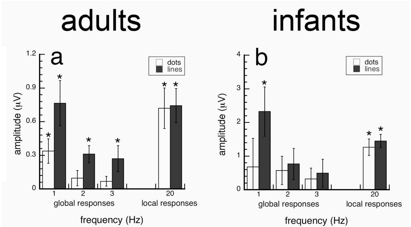
Figure 4. Projected amplitudes of local (20 Hz) and global responses (1–3 Hz) to Glass and line patterns with a 49.6 separation/length for texture flows that alternated between horizontal to random global organizations. Adults and infants showed significant responses to the global structure of line patterns, but only adults showed significant responses to the global structure of Glass patterns. Local responses to the dot and line elements were also significant in infants and adults. Error bars represent \pm SEM. *p-value<0.05, **p-value<0.001 two-tailed two-sample t-test.
