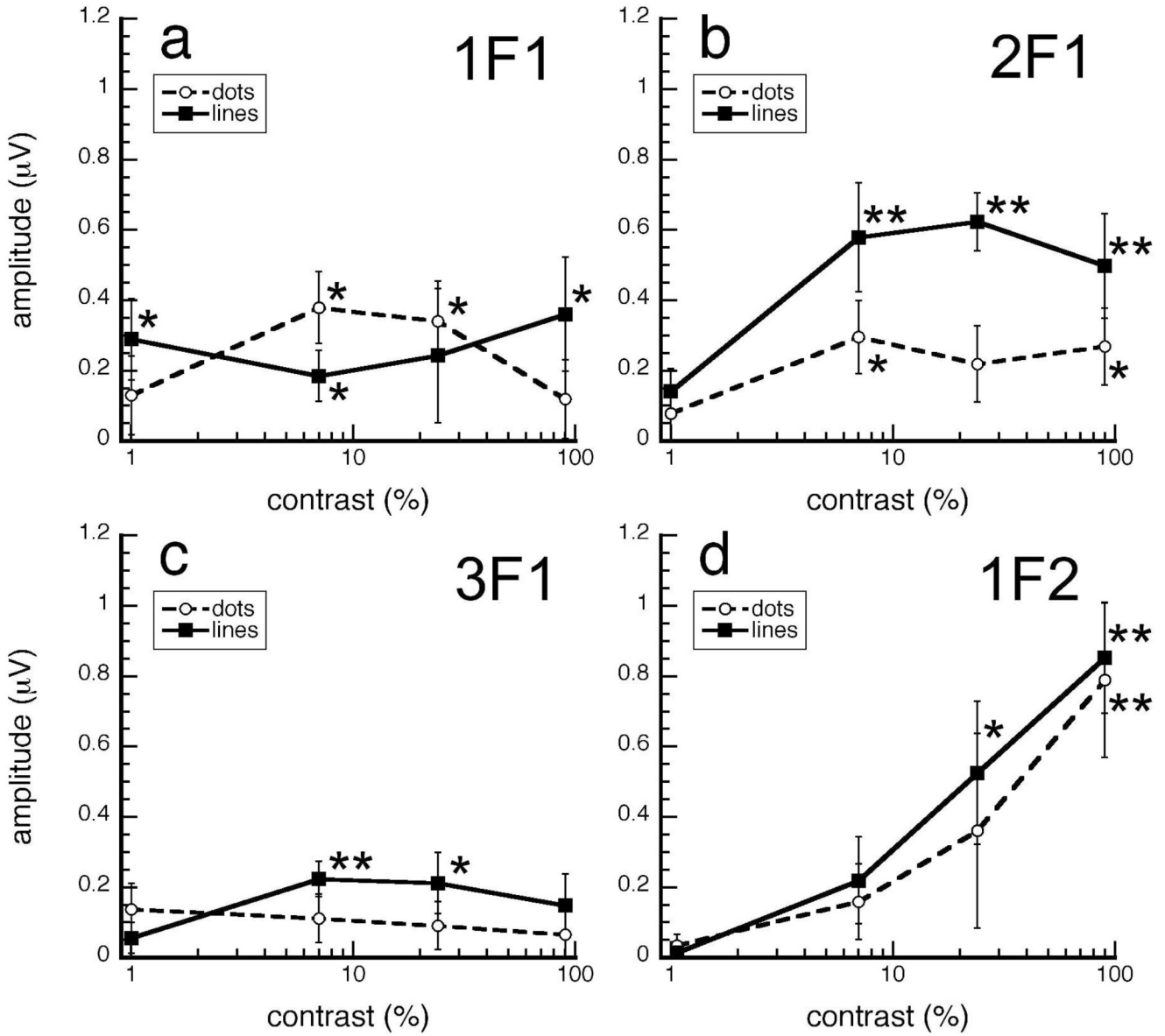
Figure 7. Projected amplitudes as a function of luminance contrast in adults. Global responses were primarily unaffected by changes in luminance contrast, whereas local responses were greatly affected. If infant insensitivity to global structure of Glass patterns is primarily caused by poorer contrast sensitivity, then adult sensitivity should be eliminated at 30% (arrow), the luminance contrast used in Expts. 1–2 reduced by a factor of 3. Error bars represent \pm SEM. *p-value<0.05, **p-value<0.001 two-tailed two-sample t-test.
