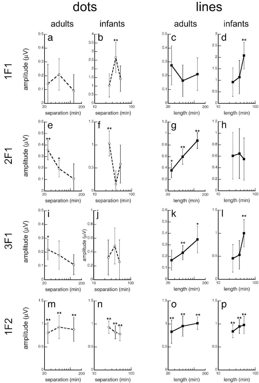
Figure 6. Projected amplitudes as a function of [LEFT] dot pair separation and [RIGHT] line length. Infants and adults show a similar trend -- global responses decreased with dot pair separation and increased with line length. However, infants have shorter interpolation spans than adults such that global responses were only significant when dot pair separation is <49.6 min. Error bars represent ±SEM. *p-value<0.05, **p-value<0.001 two-tailed two-sample t-test.
