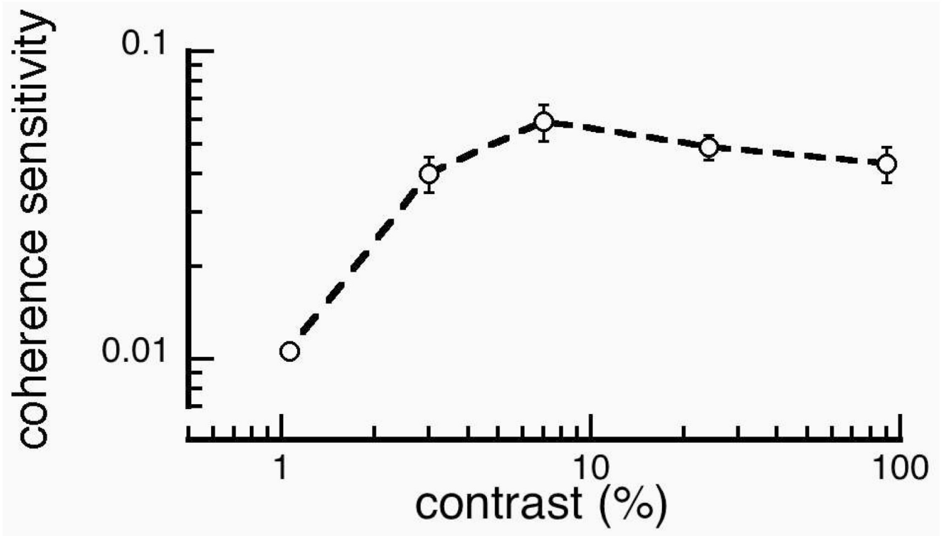
Figure 8. Geometric mean of psychophysical coherence sensitivity as a function of luminance contrast in adults. Thresholds are plotted as the inverse of the percentage of coherent elements. Once the dots are visible, sensitivity is invariant to luminance contrast. Error bars represent \pm SEM.
