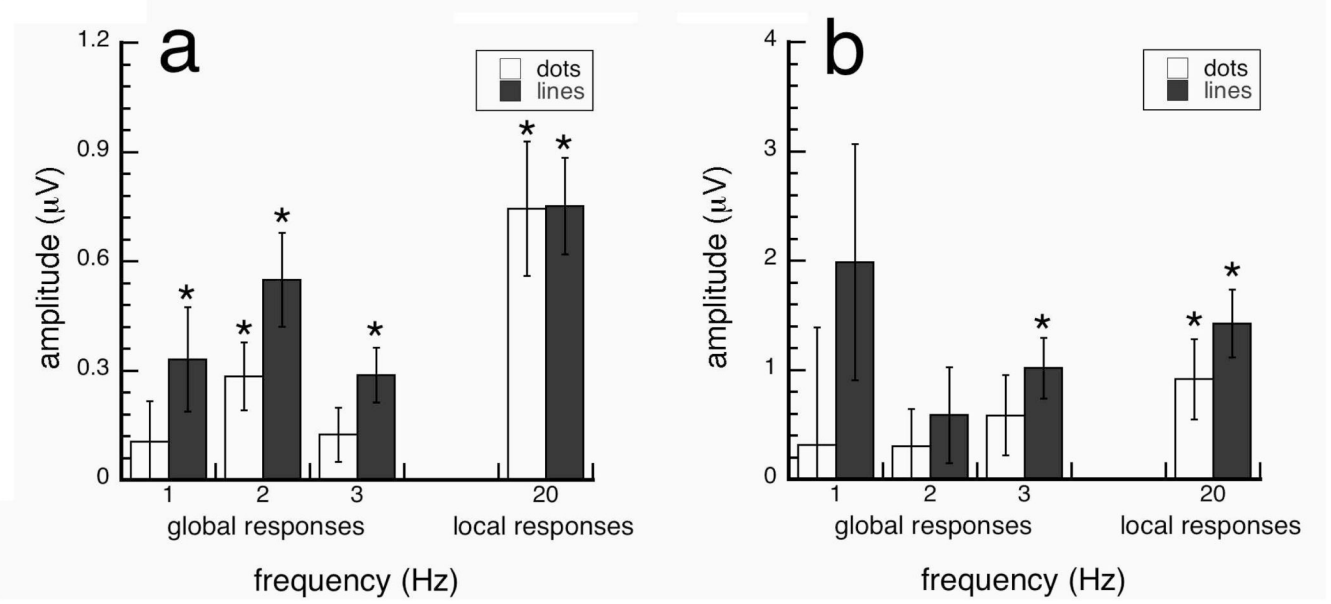
Figure 5. Projected amplitudes of local (20 Hz) and global responses (1–3 Hz) to Glass and line patterns with a 49.6 separation/length for texture flows that alternated between horizontal and co-circular organizations. Adults and infants showed significant responses to the global structure of line patterns, but only adults showed significant responses to the global structure of Glass patterns. Local responses to the dot and line elements were also significant in infants and adults. Error bars represent \pm SEM. *p-value<0.05, **p-value<0.001 two-tailed two-sample t-test.
