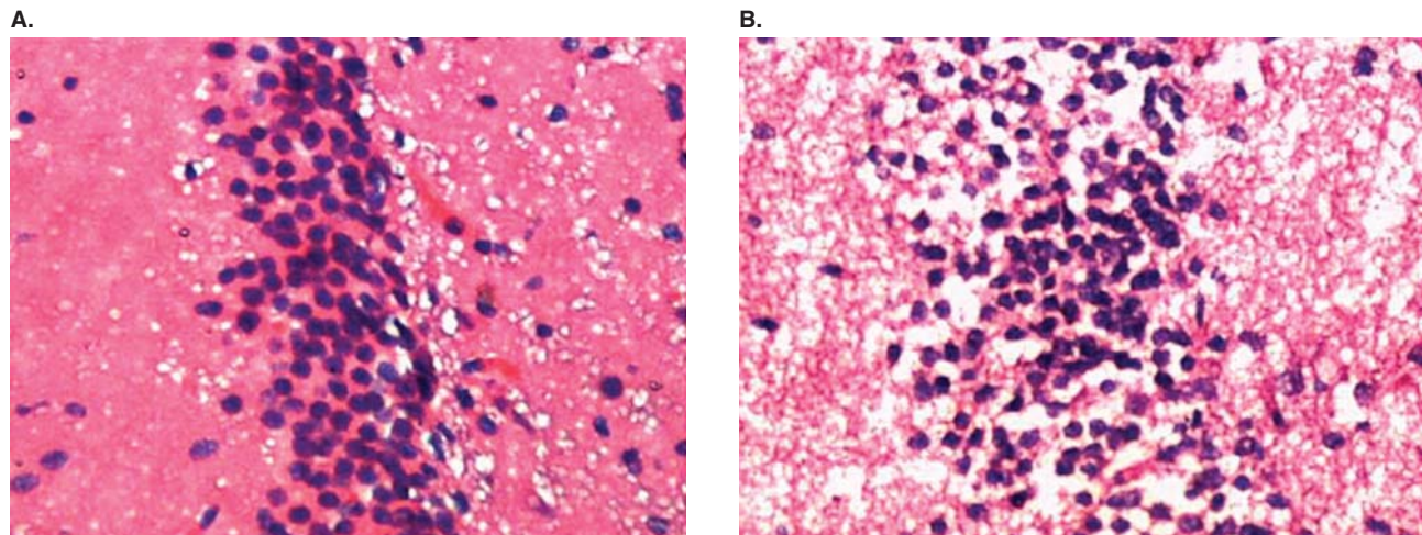
Figure 3. Representative photomicrograph of sections of hippocampal CA 3 region of the brain from both control and radio-frequency electromagnetic radiation (RF-EMR)-exposed rat stained with hematoxylin and eosin. A: Control animal; row of normal nerve cells in a section of the pyramidal cell band of the hippocampus CA 3 region is seen. B: Mobile phone RF-EMR-exposed rat; among the normal nerve cells, dark (deeply stained) and shrunken nerve cells are seen.
