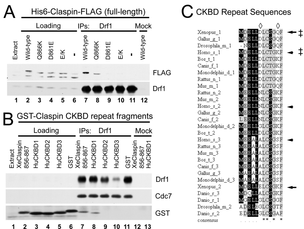
FIGURE 3. Identification of conserved sites in Claspin required for interaction with DDK. A , interphase, nuclei-free egg extracts containing full-length versions of wild-type His 6 -Claspin-FLAG, His 6 -Claspin-FLAG-Q866K, His 6 -Claspin-FLAG-D861E, His 6 -Claspin-FLAG-E/K, or no recombinant protein were immunoprecipitated with anti-Drf1 antibodies (lanes 7–11). Extracts containing wild-type His 6 -Claspin-FLAG were also mock immunoprecipitated with control antibodies (lane 12). Lanes 2–6 depict 2% of the pre-IP extracts supplemented with the recombinant proteins listed above. Lane 1 shows an aliquot of interphase extract alone. The immunoprecipitates were immunoblotted with anti-FLAG and anti-Drf1 antibodies. B , interphase, nuclei-free egg extracts containing GST-XeClaspin(856–867), GST-HuClaspin-CKBD1, GST-HuClaspin-CKBD2, GST-HuClaspin-CKBD3, and GST were immunoprecipitated with anti-Drf1 antibodies (lanes 7–11). Extracts containing GST-Claspin(856–867) and GST-HuCKBD1 were also mock immunoprecipitated with control antibodies (lanes 12 and 13). Lane 1 contains an aliquot of pre-IP interphase extract, and lanes 2–6 depict 2% of the pre-IP extracts supplemented with the recombinant proteins listed above. The immunoprecipitates were immunoblotted for Drf1, Cdc7, and GST. C , a sequence alignment of the CKBD repeat sequences across a selection of metazoan Claspin homologs. The organisms represented here are X. laevis (South African claw-toed frog), Gallus gallus (domestic chicken), Drosophila melanogaster (fruit fly), Homo sapiens (human), Bos taurus (domestic cow), Canis familiaris (domestic dog), Monodelphis domestica (gray short-tailed opossum), Rattus norvegicus (Norway rat), Mus musculus (house mouse), and Danio rerio (zebrafish). The arrows point to the X. laevis Claspin CKBD repeats, and the arrowheads point to the H. sapiens CKBD repeats. Asterisks denote positions that are conserved in all CKBD repeats. Diamonds indicate crucial residues for binding of DDK, and crosses denote the CKBD repeats in X. laevis and H. sapiens that associate with DDK.
