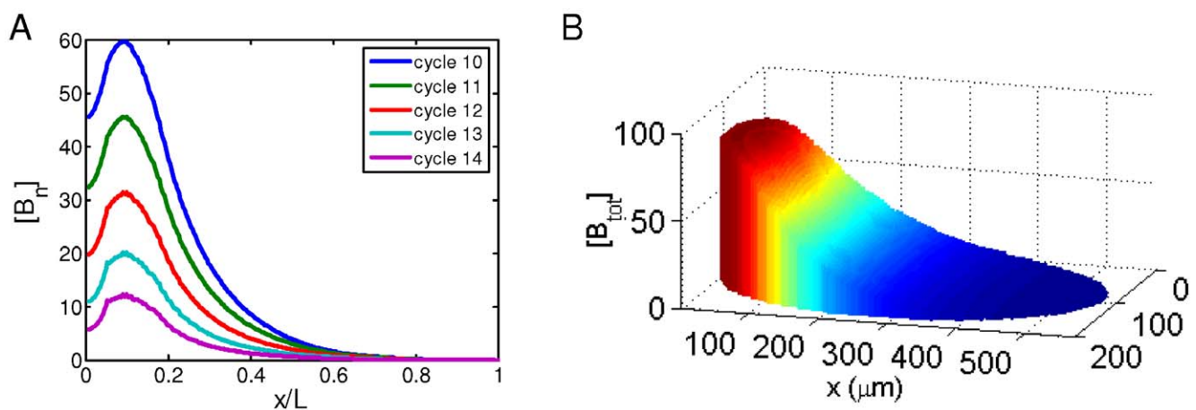
Figure 5. The effects of K_A on simulated Bcd gradient properties. A. A plot of [B_n] at nuclear cycles 10–14 in a simulation in which K_A = 10^7 \text{ M}^{-1} . This figure is the same as Fig. 2B, except the difference in K_A values used in simulations ( K_A = 5 \times 10^5 \text{ M}^{-1} for Fig. 2B). Note the instability of [B_n] profiles between different nuclear cycles ( g = -0.3557 ) and a reduction in length constant ( \lambda/L = 0.12 at nuclear cycle 14) in this simulation. B. A simulated embryo showing [B_{tot}] at nuclear cycle 14. This figure is the same as Fig. 1A except that different K_A values are used in simulations ( K_A = 10^4 \text{ M}^{-1} for this figure and K_A = 5 \times 10^5 \text{ M}^{-1} for Fig. 1A). Note a lack of cortical layer enrichment of Bcd molecules in this simulation, with a ratio of total Bcd molecules in the cortical layer to those in the inner part of the embryo, Ratio = 0.6328 . doi:10.1371/journal.pone.0010275.g005
