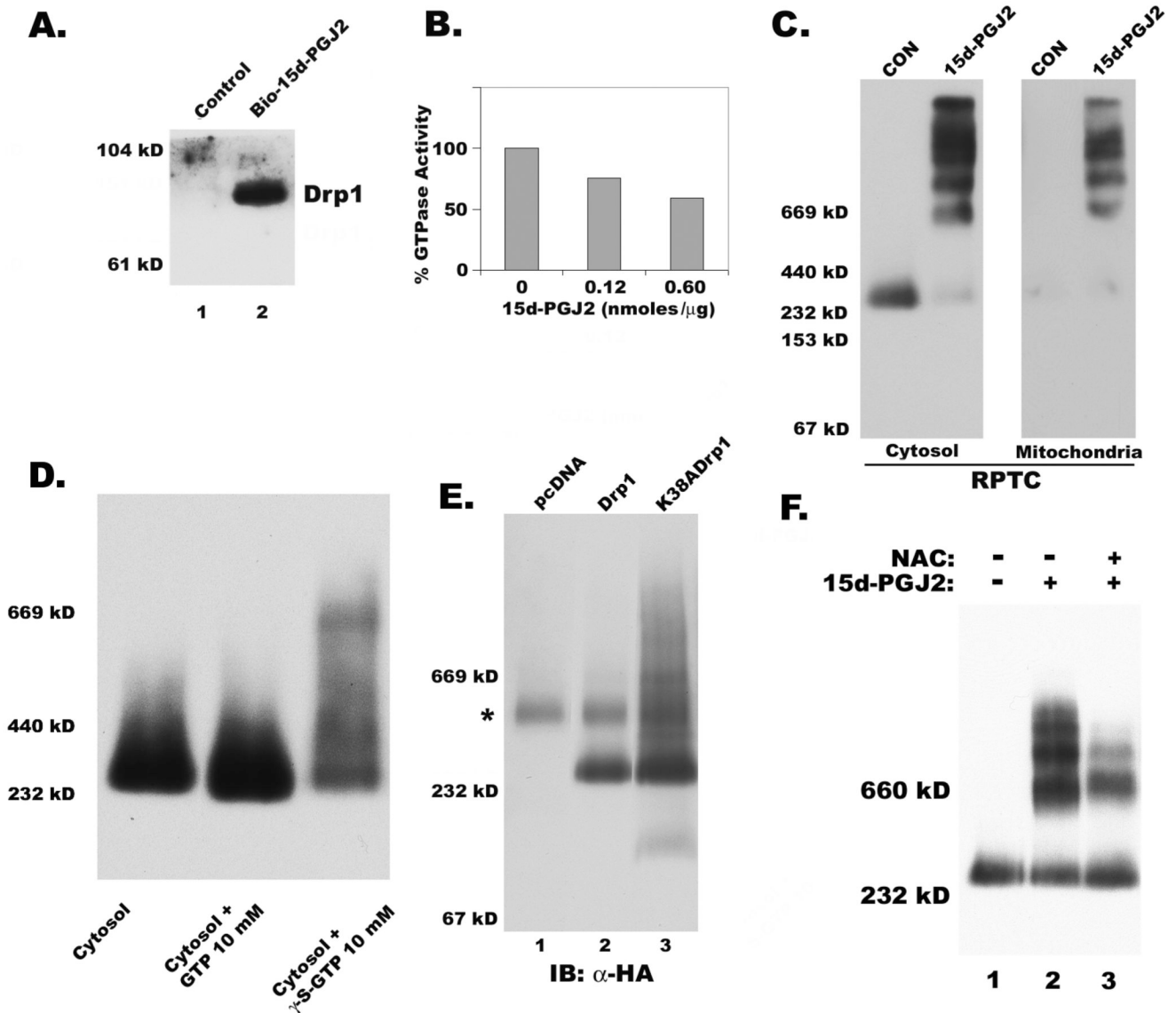
Figure 3. Covalent binding by 15d-PGJ2 and inhibition of GTPase activity resulted in oligomerization of Drp1
