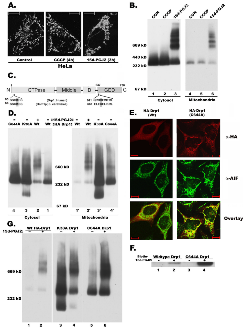
Figure 4. C644A GED domain mutation is similar to K38A GTPase inactive mutation in causing mitochondrial elongation
