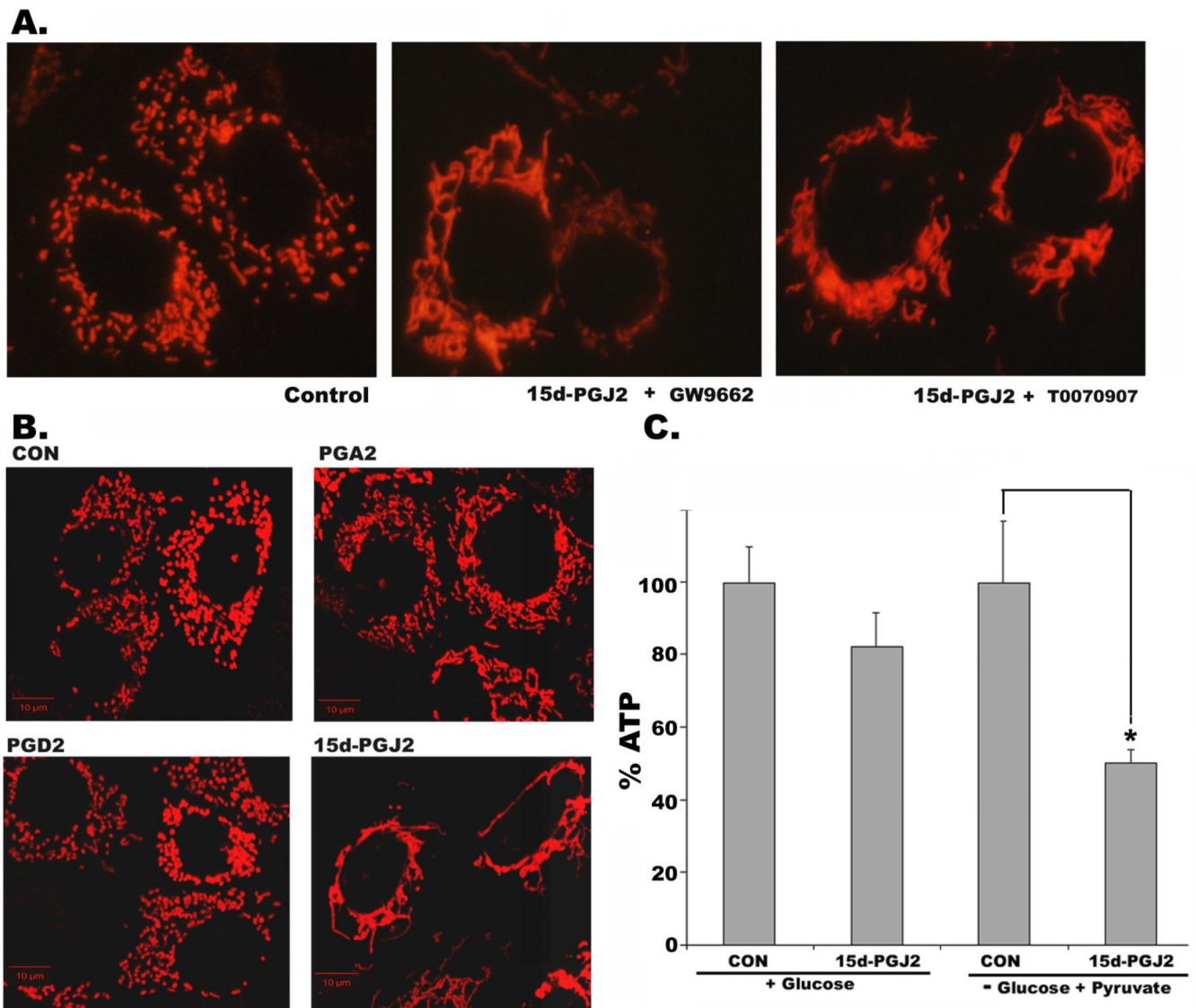
Figure 2. 15d-PGJ2 induced changes in mitochondrial morphology are PPAR \gamma independent and are unique to 15d-PGJ2 that leads to decreased ATP production
