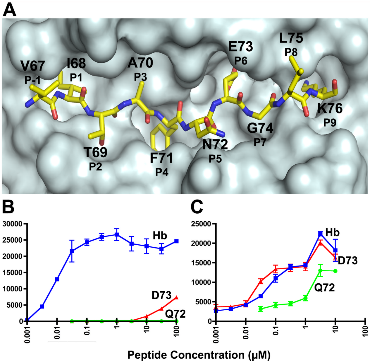
Fig. 1. T cell response of the 3.L2 T cell and the high-affinity M15. A. A top view of the surface of the crystal structure of Hb/I-E k showing the anatomy of the Hb peptide. A surface was generated for the I-E k molecule without the Hb peptide, and then a representation of the Hb peptide was superimposed onto the surface. Each amino acid position of the peptide is designated by the amino acid using the one letter code, the residue number found in the Hb protein chain, and standard peptide register number. There are 4 MHC anchor residues (P1, P4, P6, and P9) and 4 TCR contact residues (P2, P3, P5, and P8). B. The response of the 3.L2 T cell to Hb, D73, and Q72, and C. the response of M15 to Hb, D73, and Q72. T cell hybridoma cells were stimulated by indicated peptide concentrations for 24 hours in the presence of CH27 antigen presenting cells. The level of stimulation was assayed by 3 H-TdR incorporation into the IL-2 dependent cell line, CTLL-2. The values represent the mean ± triplicate values. Representative experiments of > 3 are shown. Please note, we have
