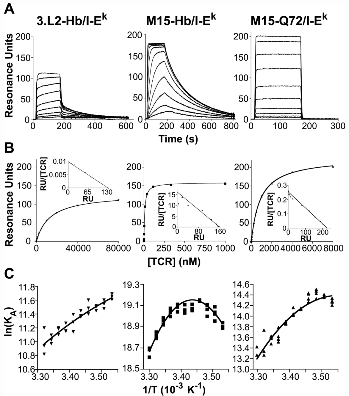
Fig. 2. Kinetic and thermodynamic features of 3.L2 and M15 scTCR binding to pMHC. Concentration series of the 3.L2 and M15 scTCRs were injected over a Biacore CM5 SPR chip surface with immobilized pMHC molecules to determine binding kinetics and K_D values. A. Sample SPR sensorgrams used to determine binding kinetic parameters of the 3.L2-Hb/I-E k interaction (left, [3.L2] are 80, 40, 20, 10, 5, 2.5, 1.25, 0.625, and 0.313 \mu\text{M} from top to bottom), M15-Hb/I-E k interaction (middle, [M15] are 500, 250, 125, 62.5, 31.3, 15.6, 7.8, 3.9, 1.95 and 0.98 nM from top to bottom) and the M15-Q72/I-E k interaction (right, [M15] are 8, 4, 2, 1, 0.5, 0.25, 0.125, 0.063, 0.032 and 0.016 \mu\text{M} from top to bottom). Sensorgrams shown are representative of three to six experiments. B. Equilibrium binding
