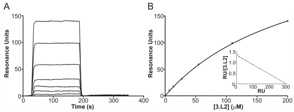
Fig. 4. Validation of the kinetics and binding affinity of the 3.L2-D73/I-E k interaction. A. Sample SPR sensorgram used to determine kinetic binding parameters for the 3.L2-D73/I-E k interaction ([3.L2] are 200, 109.5, 54.8, 27.4, 13.7, 6.9, and 3.5 μM from top to bottom). Sensorgram shown is representative of four experiments. B. Equilibrium binding analysis of the 3.L2-D73/I-E k interaction to determine the equilibrium K_D . Data are presented as the mean \pm standard deviation, and plots are representative of four experiments.
