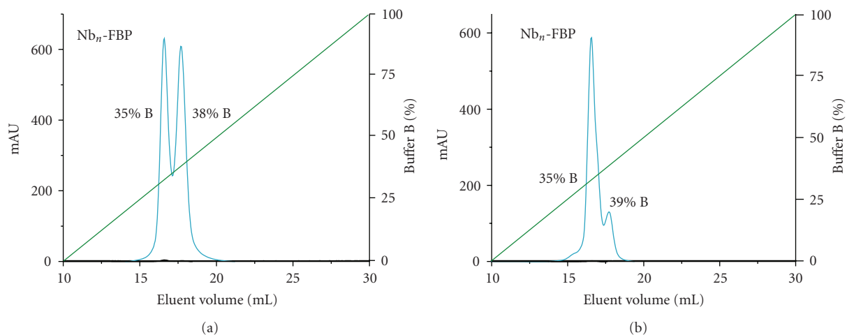
FIGURE 6: Characterization of \text{Nb}_n\text{-Fbp} (apo-Fbp reloaded with [\text{Cp}_2\text{Nb}(\text{OH})\text{Cl}_2] (a) or [\text{Nb}(\text{NTA})_2]^- (b)) by chromatography on a MonoS HR 5/5 column. The left axis shows the absorption profile at 280 nm, and the right axis is the percentage of buffer B (10 mM Hepes, 1 M NaCl, pH7.5). Green line: gradient of the buffer B applied during the elution process; cyan line: absorbance at 280 nm.
