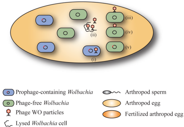
(a) Phage Transfer Between Coinfecting Wolbachia
