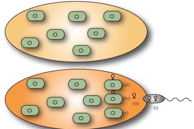
(b) Paternal Phage Transmission
