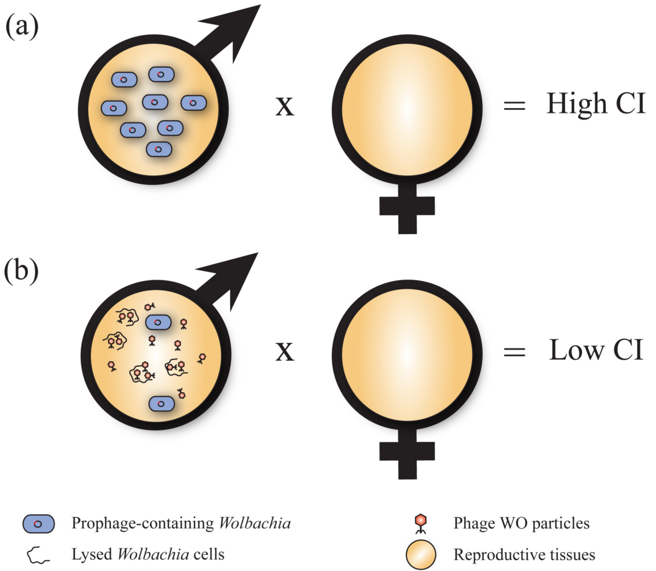
Figure 3. The phage density model of cytoplasmic incompatibility (CI). (a) When phage WO is lysogenic and titers of Wolbachia are high in male reproductive tissues, high levels of CI prevent the production of viable offspring after mating with an uninfected female. (b) When phage WO in these Wolbachia becomes lytic, Wolbachia cell titers decrease due to cell lysis and cause the infected male and uninfected female to produce an increased number of offspring [27].
