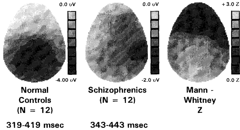
Fig. 3. Topographic distribution of N400 component activity (319–419 ms in normal controls and 343–443 ms in schizophrenics) and Mann-Whitney Z-SPM. Left and middle panels: These voltage maps show that normal controls produced a relatively symmetrical pattern of negativity (darker greys equal greater negativity), with a posterior minima at the midline. By contrast, schizophrenics showed a slightly greater negativity over right scalp than left. Grey-coded voltages are scaled differently for schizophrenics and normal controls to make scalp distributions clearly visible. Voltage scale maxima and minima are the following: normal controls = 0.0 to -4.0 \mu\text{V} ; schizophrenics = 0.0 to -2.0 \mu\text{V} . Right panel, SPM: scale maxima and minima were the following: Z = +3.0 to 0.0. The largest Z-values were in the left temporal-occipital scalp region (TCPI, P3, O1) with Z-values ranging from 2.02 to 2.60. The Z-values of neighboring centro-temporal electrodes (T3, C3, Cz, C4, T4) were 0.02 to 1.76.
