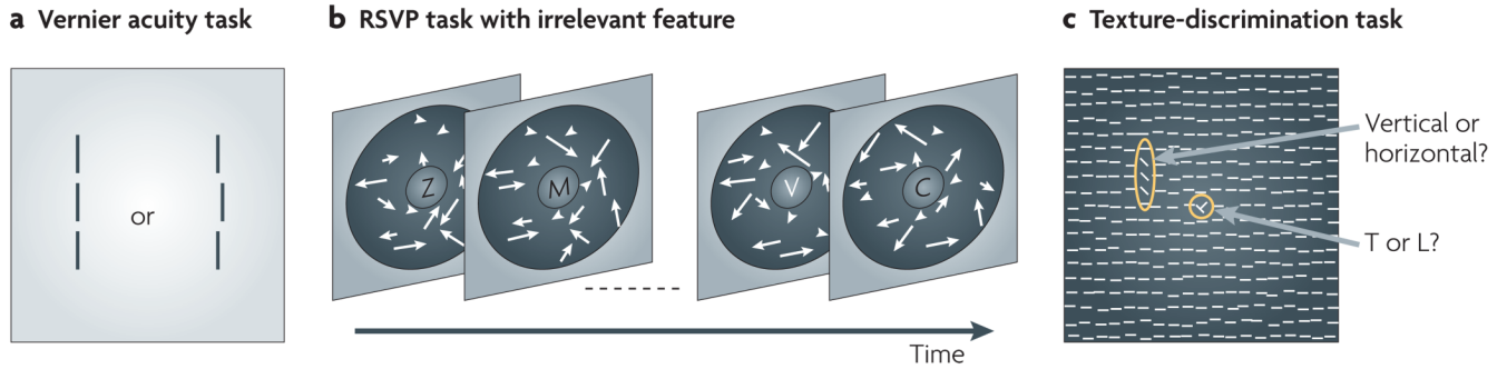
Figure 2. Typical tasks used in VPL studies
