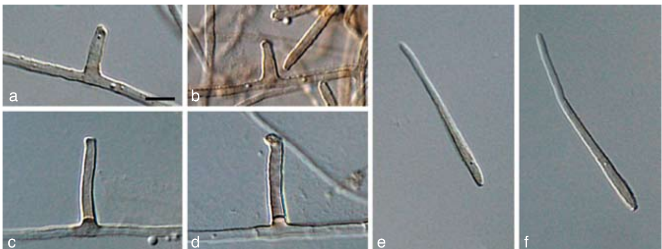
Fig. 13 Stenella musae (CBS 122477). a–d. Conidiophores with sympodially proliferating conidiogenous cells; e–f. conidia. — Scale bar = 10 \mu m.
