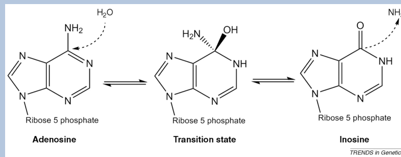
Figure I. Mechanism of adenosine deamination
