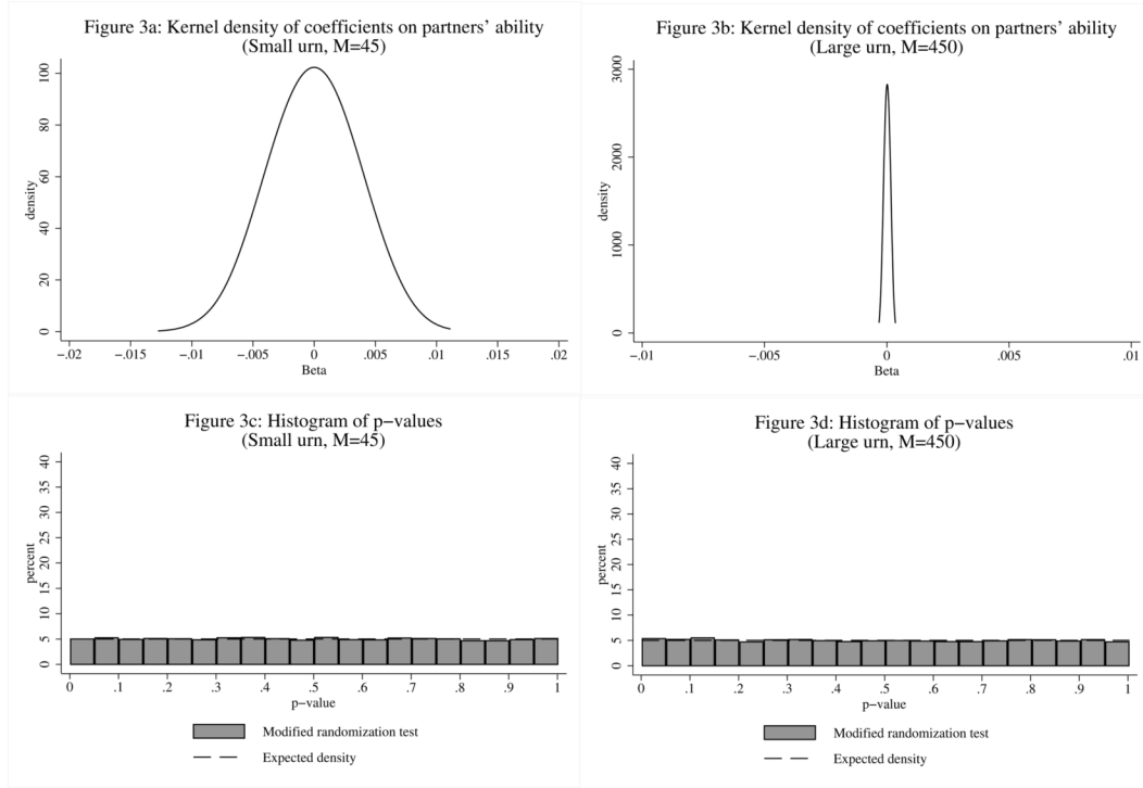
Figure 3. Monte Carlo of Modified Randomization Tests
