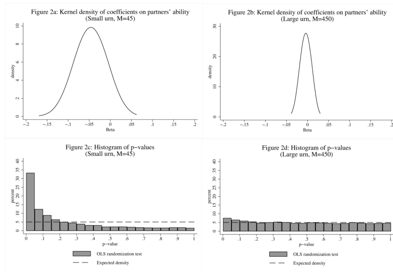
Figure 2. Monte Carlo of OLS Randomization Tests
