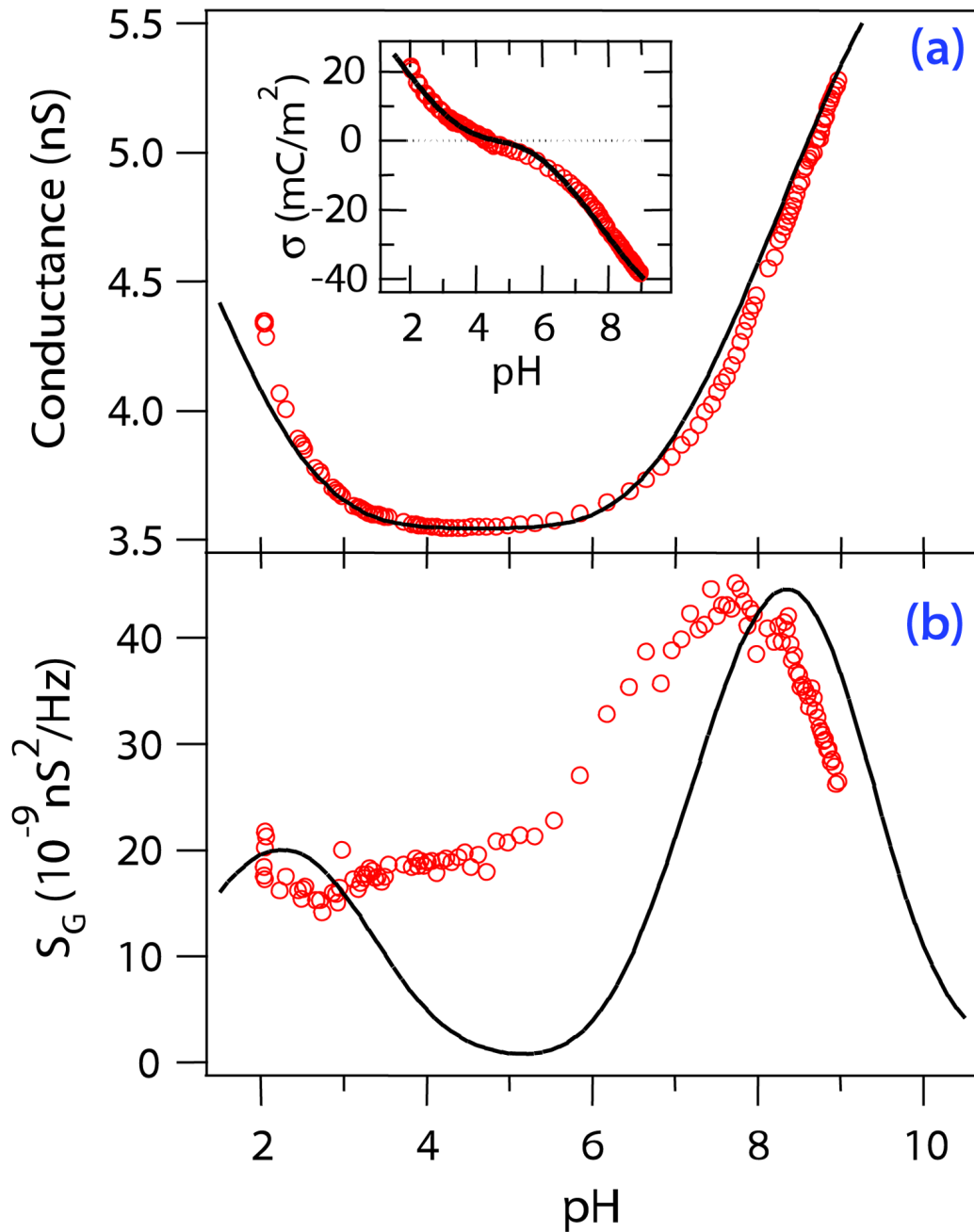
FIG. 3. (color online). (a) Measured conductance (open circles) vs pH at constant 110 mM ionic strength. The minimum at pH \sim 4.1 corresponds to the point of zero charge. The solid line represents the predicted conductance from a fluctuating 3-level system. Inset: Surface charge as induced from the data (open circles) and as predicted by the model (solid line). (b) Experimental noise spectral density (open circles) vs pH . The solid line is a fit to the charge fluctuation model presented in the text. Both curves are modeled by the same set of parameters that was used to fit the variable electrolyte concentration data (see Fig. 2).
