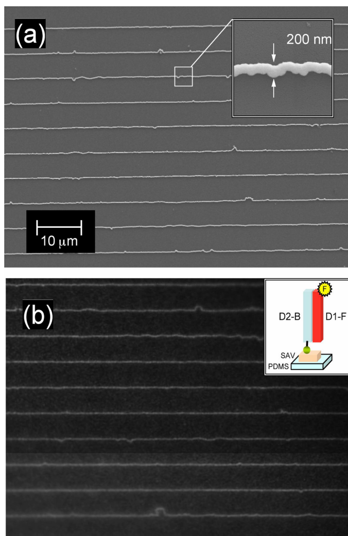
Figure 2. SEM image of a gold nanowire array master and fluorescence image of DNA nanolines on PDMS replica. (a) A representative large area scan showing a portion of gold nanowire array with average spacing of 5 μm. The inset is a high-magnification image of a single gold nanowire with an average width of 200 nm. (b) A 60x fluorescence image of the PDMS replica surface obtained after the master-replica transfer process and exposure to D1-F, a fluorescently labeled ssDNA complementary to D2-B. The inset is a schematic diagram of the replica surface.
