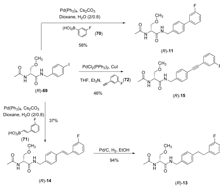
Scheme 6. Preparation of Compounds (R)-11, (R)-13, (R)-14 and (R)-15
