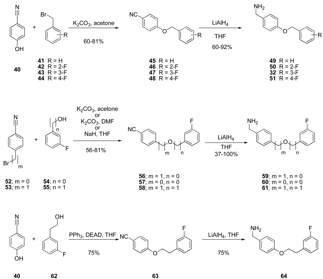
Scheme 4. Benzylamine 32 , 49–51 , 59–61 , and 64 Synthesis
