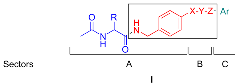
Figure 1. Overlay of Pharmacophores in I
