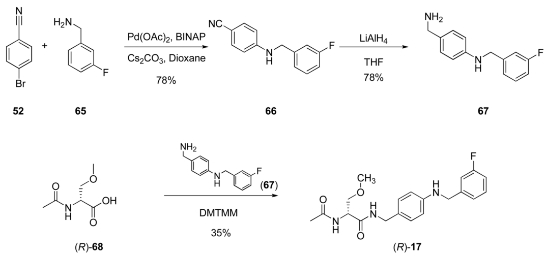
Scheme 5. Benzylamine 67 and Compound (R)-17 Synthesis
