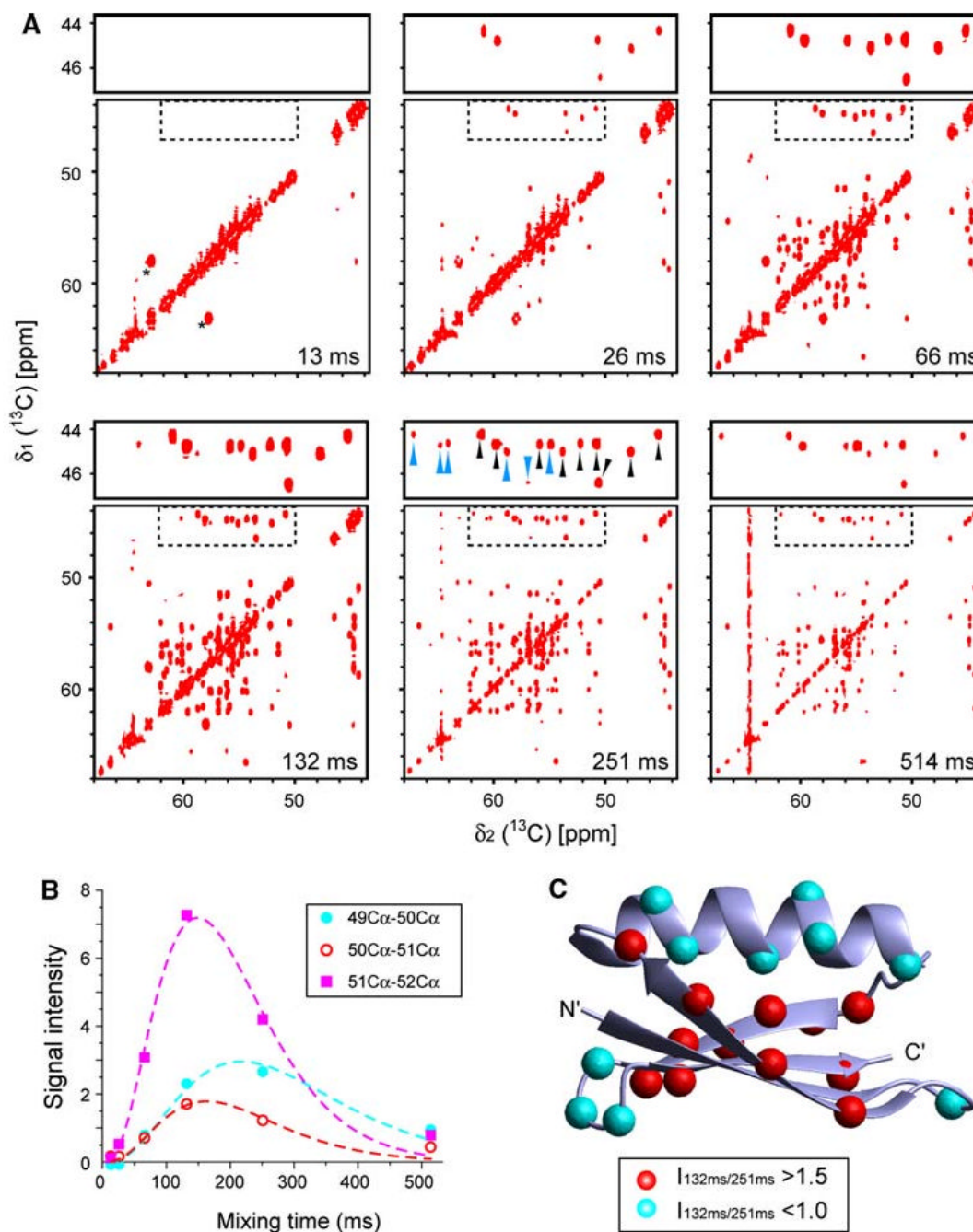
Fig. 2. Mixing efficiency of the CACA-TOCSY experiment with [\text{U-}^2\text{H}, ^{15}\text{N} + 2\text{-}^{13}\text{C}] -GB1 (5 mM) recorded in 20% glycerol at 285 K, which corresponds to a 90 kDa protein in aqueous solution at room temperature. a The CACA-TOCSY spectra at various mixing times ranging from 13 to 514 ms. As easily analyzable areas, the regions containing correlations to glycine residues ( dotted square ) are enlarged on top of each spectrum. Black and cyan arrow heads in the enlarged section at 251-ms mixing time indicate sequential and long range ( i:i-2 or i:i+2 ) correlations between \text{C}^\alpha nuclei, respectively. The measuring time for each spectrum was 5.5 h. The black asterisks in the 13 ms mixing time spectrum denote signals arising from natural abundance ^{13}\text{C} -nuclei of glycerol. 2D CACA-TOCSY experiments were recorded with a
