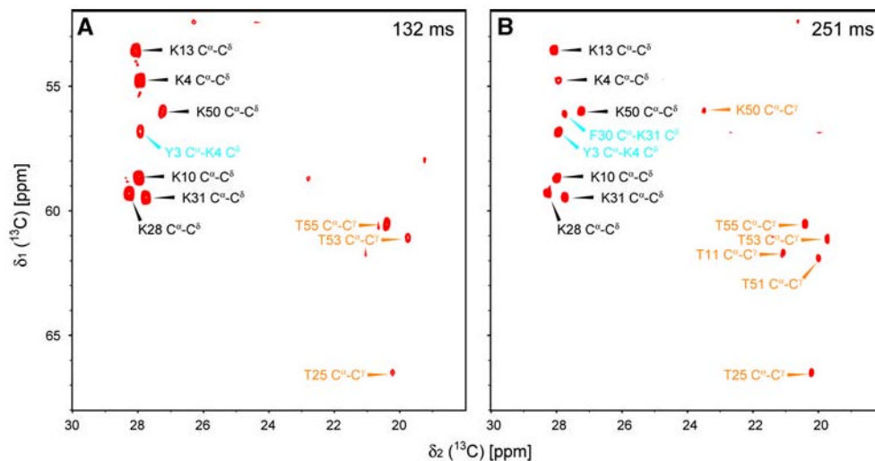
Fig. 5. C^\alpha to sidechain carbon correlations in the CACA-TOCSY experiment. The spectra were recorded with [\text{U-}^2\text{H}, ^{15}\text{N} + 2\text{-}^{13}\text{C}] -GB1 (5 mM) under the same conditions as those in Fig. 2, with mixing times of 132 ms ( a ) and 251 ms ( b ). The measuring time for each experiment was 5.5 h. Black and cyan arrowheads in the spectra indicate intra-residual and sequential C^\alpha - C^\delta correlations, respectively. Orange arrowheads are for intra-residual C^\alpha - C^\gamma correlations
