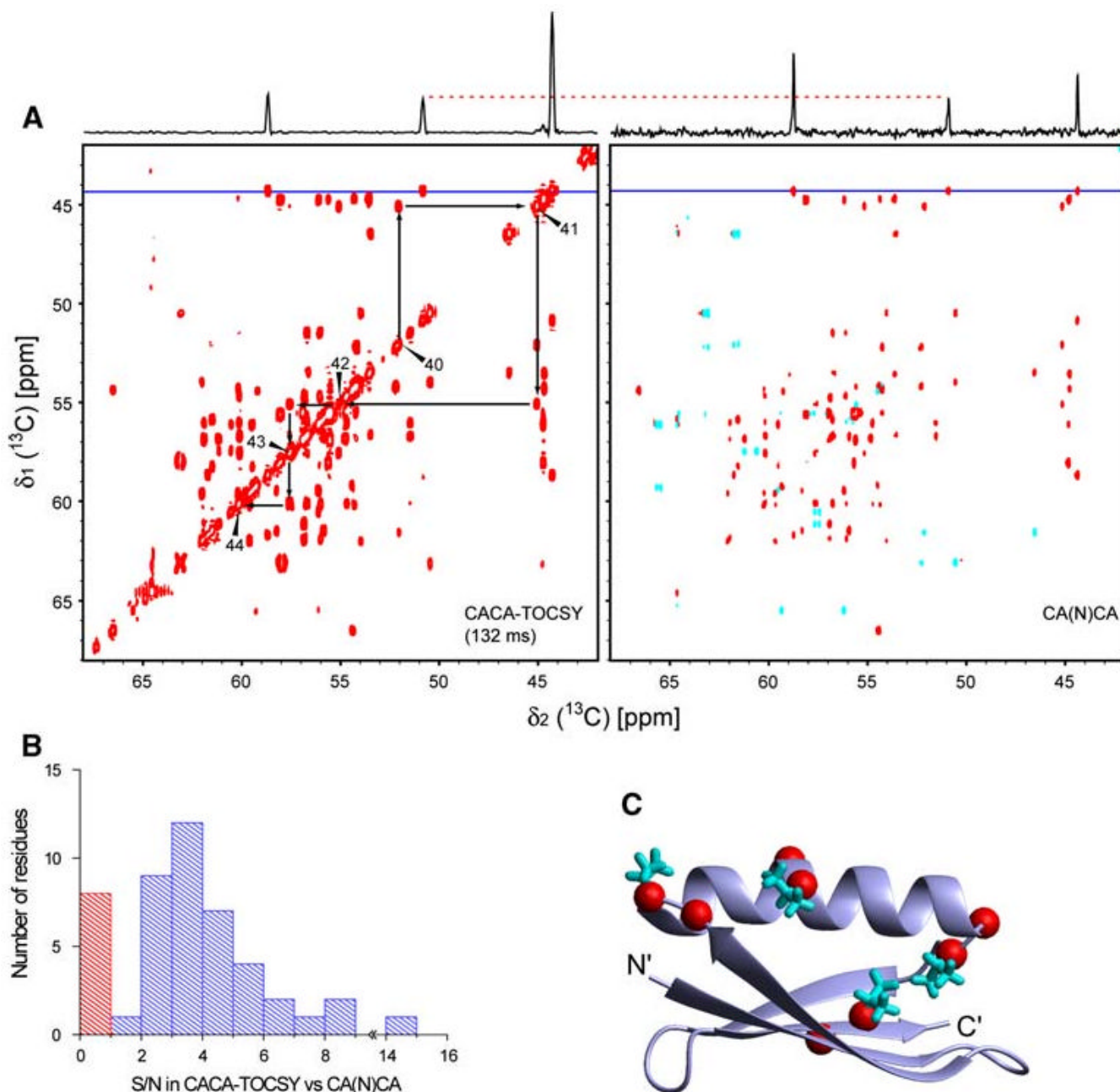
Fig. 3. Comparison between the CACA-TOCSY and CANCA experiments. a The CACA-TOCSY (132 ms) and CANCA spectra were recorded at the same condition as in Fig. 2. The measuring time for each experiment was 5.5 h. Slices at the position of the horizontal blue lines (corresponding to Gly9) are shown on top of each spectrum. The vertical scales of the slices are normalized by the peak intensity of the middle resonances originating from C^\alpha of residue Asn8. Black arrows in the CACA-TOCSY indicate the assignment walk connecting the C^\alpha of residues 40–44. Starting from C_i^\alpha diagonal at \omega(C_i^\alpha) , one can find the C^\alpha frequency of the preceding or succeeding residue \omega(C_{i-1}^\alpha or C_{i+1}^\alpha ). b Histogram of the ratios of the signal-to-noise values (S/N) in the CACA-TOCSY over the S/N in CANCA. The average of the S/N
