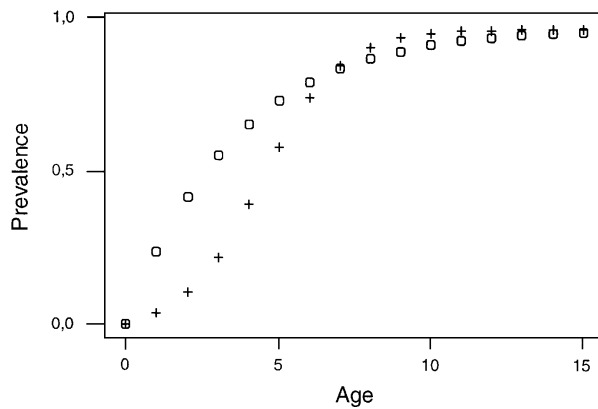
Fig. 1. Smoothed prevalence. (oooooo EXPO1 model, + + + + + LOGIS1 model)
