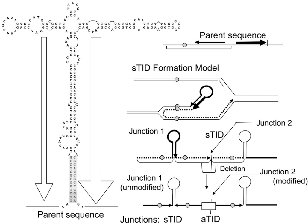
FIGURE 9.—A TID amplification with one unmodified symmetrical junction. The diagram at left and the solid arrows at top right indicate a parental quasi-palindromic sequence that might generate snap-back pairing. The events at right describe how the snap-back structure might prime repair synthesis, leading to the TID junction sequences found in strain TT25790 (Table 1). The quasi-palindromic junction is extended without modification. The second junction forms by template switching and is later modified by deletion.
