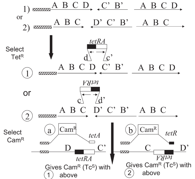
FIGURE 7.—Genetic testing of TID amplification structure. To determine whether an aTID junction is in orientation CD' or DC', a resistance determinant ( tetRA ) was added to the sequenced junction of strain TT25771 (see Table 1). The chromosome of the resulting strain is expected to be as diagrammed for strain 1 or strain 2 (circled). In a second transformation cross, a donor \text{Cam}^R determinant is introduced with one flanking sequence matching a reference region at the left and the other matching the tetRA sequence. The \text{Cam}^R determinant can be inherited only if the orientation of the recipient junction ( tetRA or ARtet ) matches that of the donor recombining sequence (right side of \text{Cam}^R ). The donor fragments are designed such that inheritance of \text{Cam}^R creates a deletion of the region between the reference sequence and the right side of the \text{Tet}^R determinant in the recipient. The recipient strain is recA + and was grown nonselectively before transformation.
