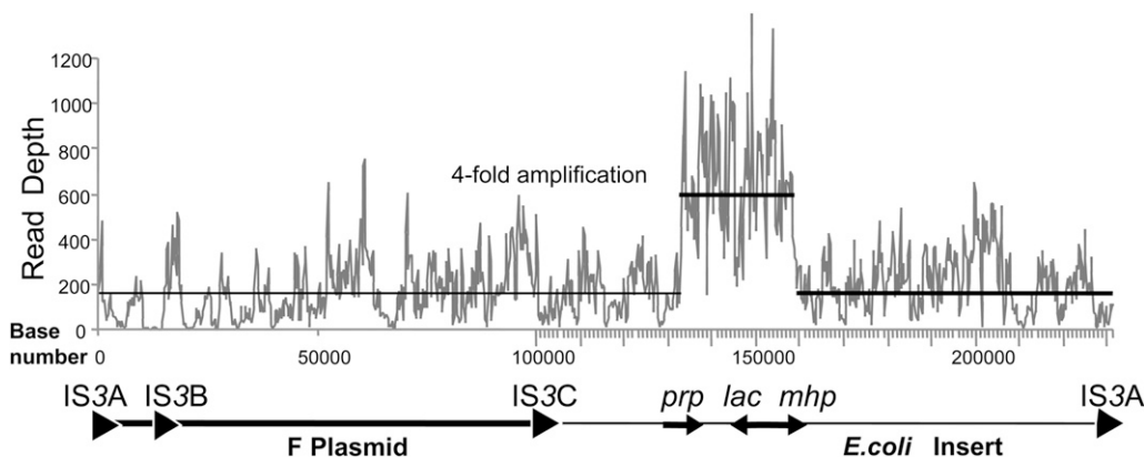
FIGURE 5.—Depth of Illumina reads from the F'_{128} lac plasmid of a strain carrying a TID amplification. The plasmid genotype is diagrammed below the graph with the F factor plasmid sequence indicated by a bold line and the E. coli material by a finer line. Strains are recA and were grown on glycerol for lac amplification. The read depth for chromosomal genes (not shown) was ~90-fold. The nearly 200-
