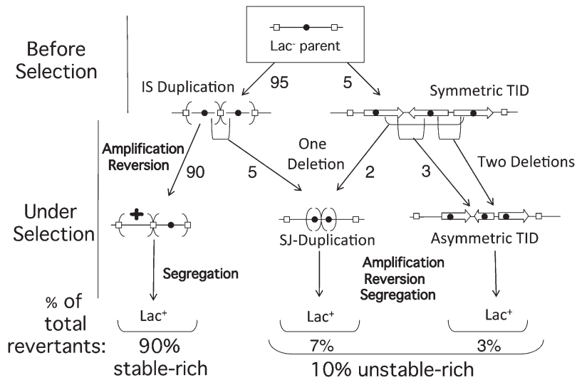
FIGURE 10.—The sTID can also contribute to formation of an SJ duplication. The parental sequence is diagrammed at the top (boxed) in which open rectangles designate a copy of IS3 and the solid circle designates the lac operon. An SJ duplication can form when a deletion removes the junction of an IS3 duplication (left middle). An SJ duplication also forms when a single deletion removes both sTID junctions (right middle). Two deletions convert an sTID to an aTID duplication. Some IS3-bounded lac duplications may form through sTID intermediates.
