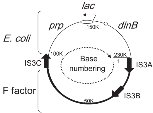
FIGURE 4.—Structure of the F'_{128} plasmid on which rearrangements occur. The base numbering conventions are the following: Bases 1–100,413 are derived from the F factor (bold arc of circle). Bases 100,414–150,235 are from the E. coli chromosome extending from IS3C to include all of the lac operon up to base 150,235, which is immediately adjacent to the promoter-proximal end of the lacZ coding sequence. Bases 150,236–231,638 of the plasmid are also from the E. coli chromosome and extend from lacZ to beginning of F factor sequence (at base 1). The origin and structure of this plasmid have been described in detail (KOFOLD et al. 2003).
