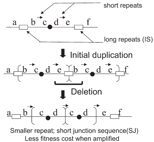
FIGURE 1.—Formation of SJ duplications under selection. The short arrows between b–c and d–e in the parent sequence are repeats of 3–12 bp. The boxes are the 1.25-kb elements IS3A and IS3C that flank lac on the F' 128 plasmid. The duplicated region between IS3 copies is ~125 kb, and duplications of this type are carried by 0.1% of cells prior to selection. Deletion between identical short sequences leaves a smaller duplication, typically ~20 kb. Shortening reduces the reversion rate and fitness cost of a duplication and thereby allows higher amplification (KUGELBERG et al. 2006).
