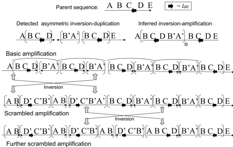
FIGURE 8.—Effects of inversions on structure of amplified aTID array. One initial aTID structure is depicted with the changes that are possible due to amplification followed by recombination between inverse-order sequence repeats.
