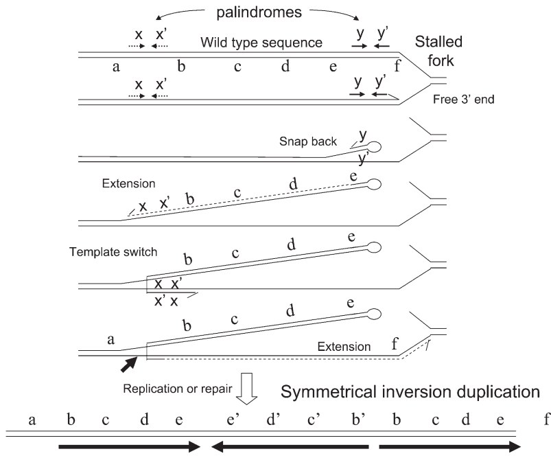
FIGURE 2.—Proposal for the formation of symmetrical TID structures. Short quasi-palindromic sequences are frequent and can support formation of snap-back structures that initiate repair synthesis, which can switch templates and be re-directed toward the fork. The resulting branched structure can be broken at arrow and repaired or can be replicated to produce the sTID structure proposed to initiate the aTID structures described here. These events may also underlie recombination-independent formation of simple duplications.
