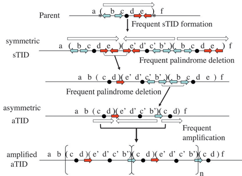
FIGURE 3.—Conversion of an sTID precursor to an aTID duplication. The sTID forms and is lost frequently. Asterisks in the parent sequence indicate small palindromic sequences that promote sTID formation. Prolonged selection for higher expression ( e.g. , lac , the black dot) favors retention of the sTID and sequential accumulation of deletions that render junctions asymmetric (forming the aTID). As fitness cost is reduced, higher amplification allows faster growth and ultimately provides sufficient lac targets so that point mutations can stably alter the gene under selection. Short colored arrows are repeated oligonucleotide sequences present in the parent that serve as endpoints for deletions and junctions of the final aTID duplication. Uninvolved repeats are omitted after the first two lines.
