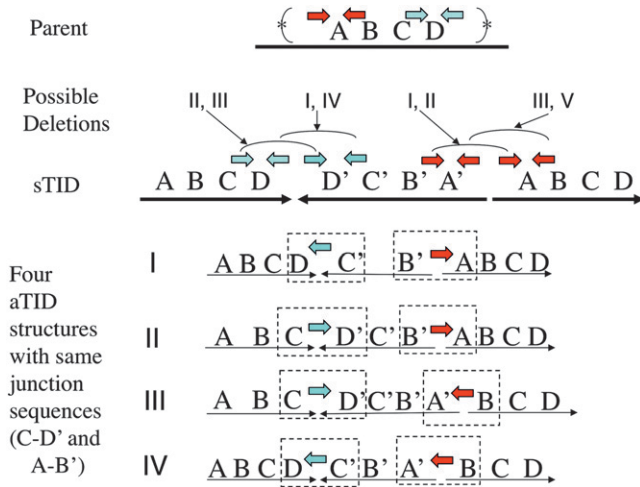
FIGURE 6.—Multiple structures are consistent with a single pair of junction sequences. In the examples listed (I–IV), the leftmost (converging) junction is D–C' (equivalent to C–D') and the rightmost (diverging) junction is B'A (equivalent to A'B). If the asymmetric inversion junctions are formed by deletions in a symmetrical precursor, then four possible structures could be generated by the various combination of deletions described in the bottom line. The colored arrows indicate repeated sequences present in inverse order in the parent chromosome and how they contribute to aTID formation.
