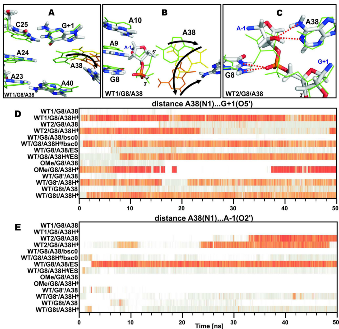
Figure 5. The canonical A38 either loses pairing with the A24 nucleobase while leaving the active site during the majority of MD simulations or, alternatively, establishes an A-1(2'-OH)...A38(N1) hydrogen bond. (A) Sticks representation of the average structure of the last ns of simulation WT1/G8/A38 illustrating the A38-A24 base pair disruption. While the crystal geometry is represented by green lines, yellow and orange lines represent snapshots of consecutive A38 positions during its expulsion (black arrow) from the active site. (B) Same as panel A, but from a different viewpoint. (C) Average structure of the active site (taken from the last ns of simulation WT2/G8/A38 and overlaid with the crystal structure in green) showing A38(N6H)...A-1(O2') and A-1(2'-OH)...A38(N1) hydrogen bond formation. (D) and (E) Time evolution of the A38(N1)...G+1(O5') and A38(N1)...A-1(O2') distances in all simulations.
