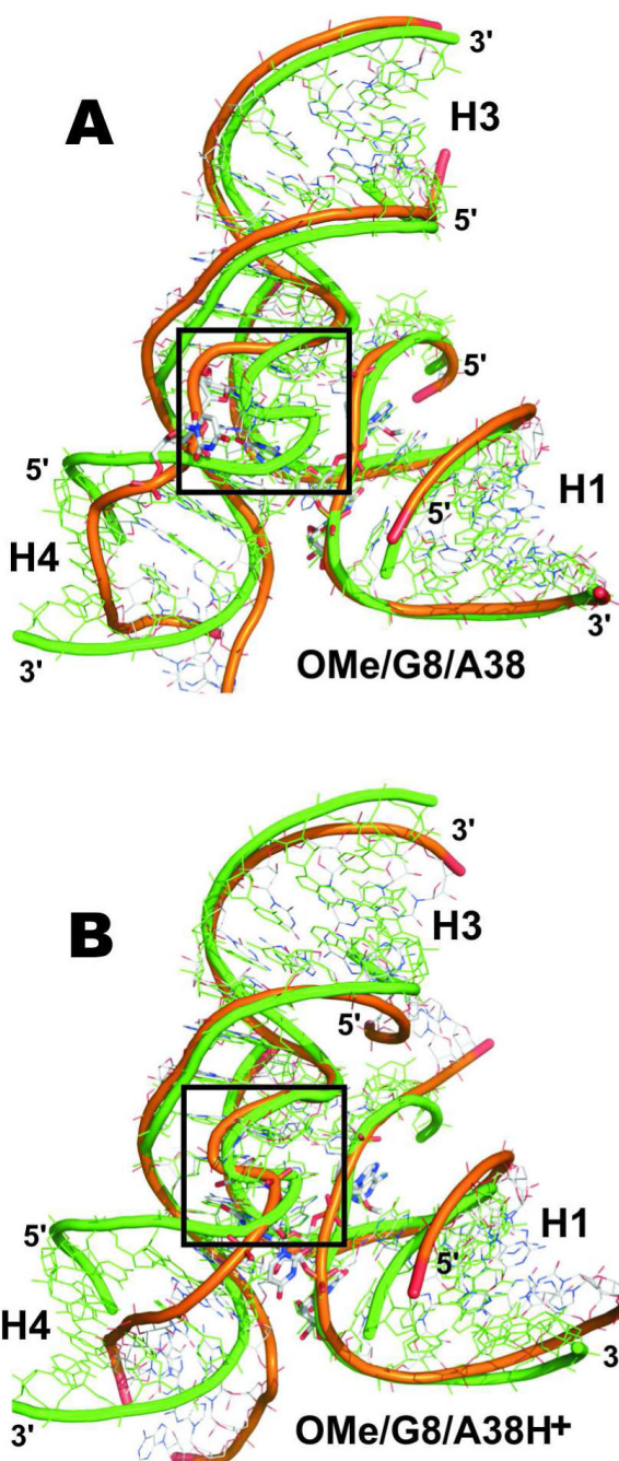
Figure 6. Ribbon diagrams showing the average structures from the last ns (orange ribbon) superimposed over the crystal structure (green) of the minimal junction-less hairpin ribozyme with helices H1-H4 indicated. (A) Simulations with canonical A38 (here OMe/G8/A38) show S-turn degradation (black box). (B) Simulations with protonated A38H + (here OMe/G8/A38H + ) preserve the crystallographic S-turn conformation.
