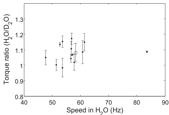
FIGURE 4 Ratio of torque in H 2 O medium to that in D 2 O medium for 13 motors at high load. Solid circles are the average of torque ratios for each motor using torques in H 2 O medium before and after the D 2 O measurement, and the error bar was calculated using the difference of torques in H 2 O medium before and after the D 2 O measurement. The open circle with the error bar is the mean \pm SD for all 13 motors ( 1.08 \pm 0.06 ).
