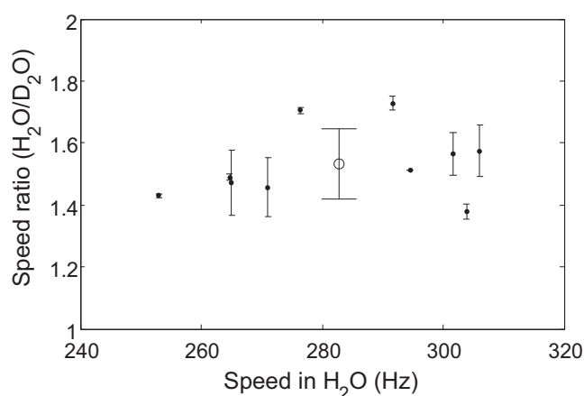
FIGURE 5 Ratio of speed in H 2 O medium to that in D 2 O medium for 10 motors near zero load. Solid circles are the average of speed ratios for each motor using speeds in H 2 O medium before and after the D 2 O measurement, and the error bar was calculated using the difference of speeds in H 2 O medium before and after the D 2 O measurement. The open circle with the error bar is the mean \pm SD for all 10 motors ( 1.53 \pm 0.14 ), including the correction for changes in the deuteron-motive force.
