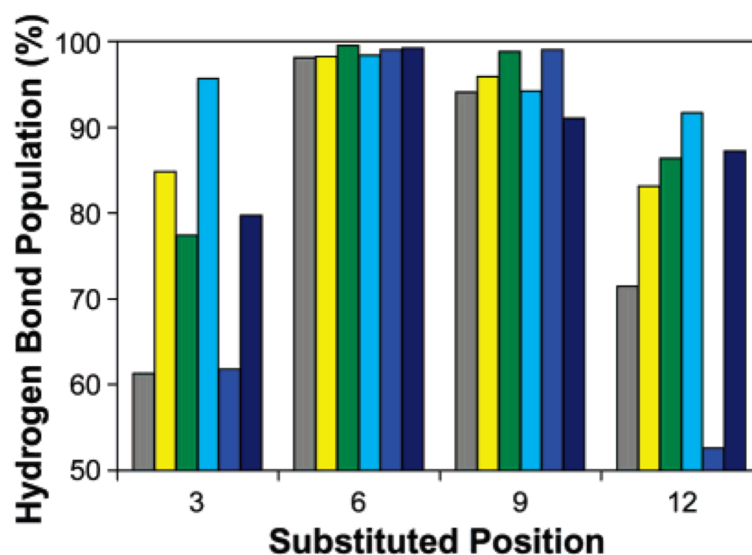
Figure 7. Hydrogen bond populations near substitution sites in Monte Carlo simulations of 14-helical oligo- \beta^3 -homoalanine peptides individually substituted at the indicated position with the following: \beta^3 -homoalanine (gray), \beta^3 -homoserine (yellow), \beta^3 -homothreonine (green), \beta^3 -homoisoleucine (cyan), \beta^3 -homoleucine (blue), or \beta^3 -homovaline (navy blue). Hydrogen bond population near a substitution site was calculated as the average population of the (i - 2 \rightarrow i) , (i - 1 \rightarrow i + 1) , and (i \rightarrow i + 2) hydrogen bonds (when available) surrounding substitution position (i) over 2 million configurations.
