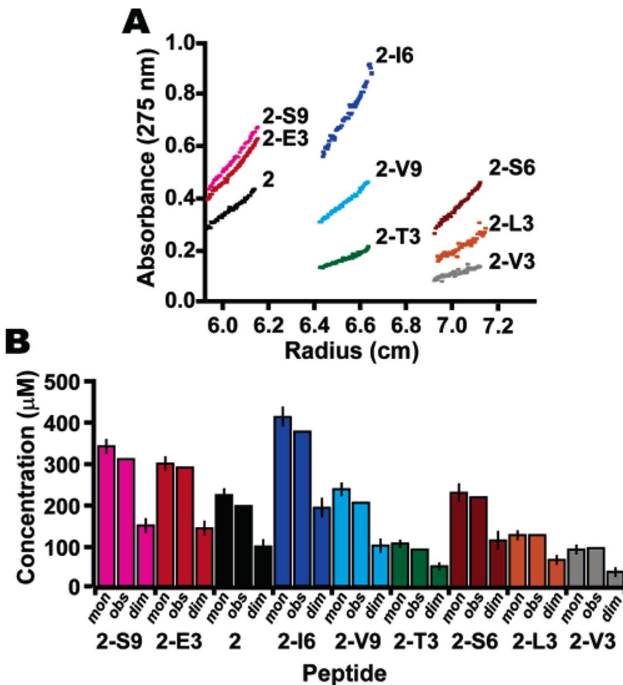
Figure 4. Analytical ultracentrifugation data (A) and material balances (B) for the following: 2-S9 (pink), 2-E3 (red), 2 (black), 2-I6 (blue), 2-V9 (cyan), 2-T3 (green), 2-S6 (brown), 2-L3 (orange), and 2-V3 (gray). Calculated concentrations are based on material balances for a monomer fit (mon) or a dimer fit (dim) to the AU data. The observed concentration is shown for comparison (obs).
