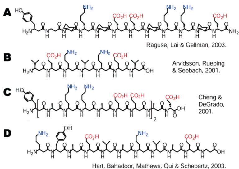
Figure 2. \beta^3 -Peptides that populate 14-helical structures in water. Coloring has been used to accentuate ( i, i + 3 ) salt-bridges. (A) \beta -Dodecamer utilizing cyclic and acyclic residues reported by Raguse et al. 20 (B) Salt-bridge-stabilized \beta^3 -heptapeptide with appreciable 14-helical CD signature in water reported by Arvidsson et al. 24 (C) Salt-bridge-stabilized 15-mer \beta^3 -peptide reported by Cheng and DeGrado. 25 (D) Macro-dipole-stabilized \beta^3 -undecapeptide reported by Hart et al. 26
