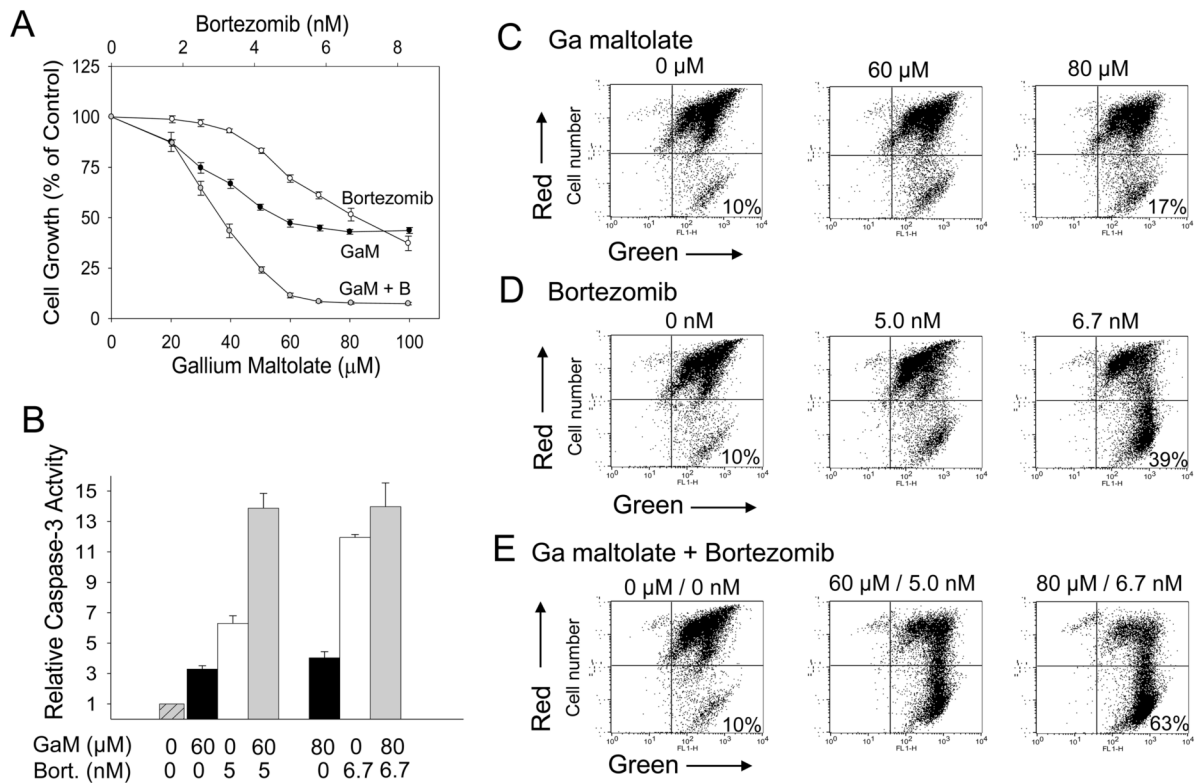
Figure 1. Bortezomib synergistically enhances gallium maltolate-induced cell in mantle cell lymphoma cells
