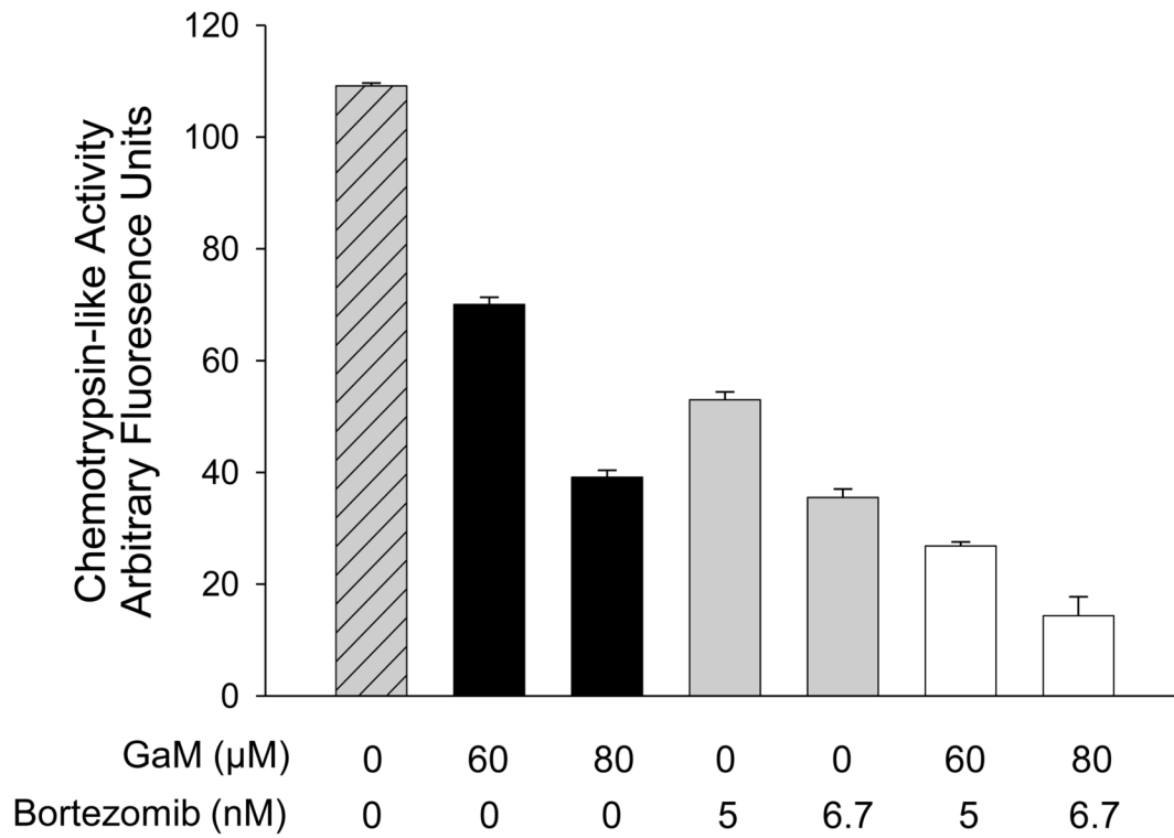
Figure 2. Inhibition of proteasome activity by gallium maltolate and bortezomib
