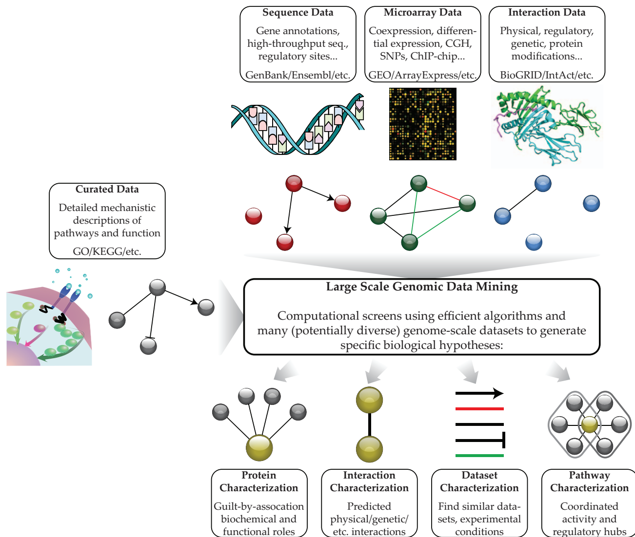
Figure 1. Large-scale genomic data mining. A schematic overview of possible inputs, data sources, network models, and output predictions from computational screens leveraging many genome-scale datasets. Note that both the “output” pathway model and the “input” experimental data are represented as networks: directed regulatory binding site targets, undirected weighted coexpression, and undirected interactions, respectively. As demonstrated by the sample analysis in Box 1, biological networks provide a uniform framework within which both experimental data and predicted models can be represented, facilitating integrative analyses. doi:10.1371/journal.pcbi.1000779.g001
