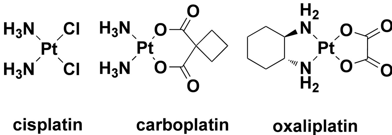
Figure 1. Chemical structures of platinum anticancer drugs.
