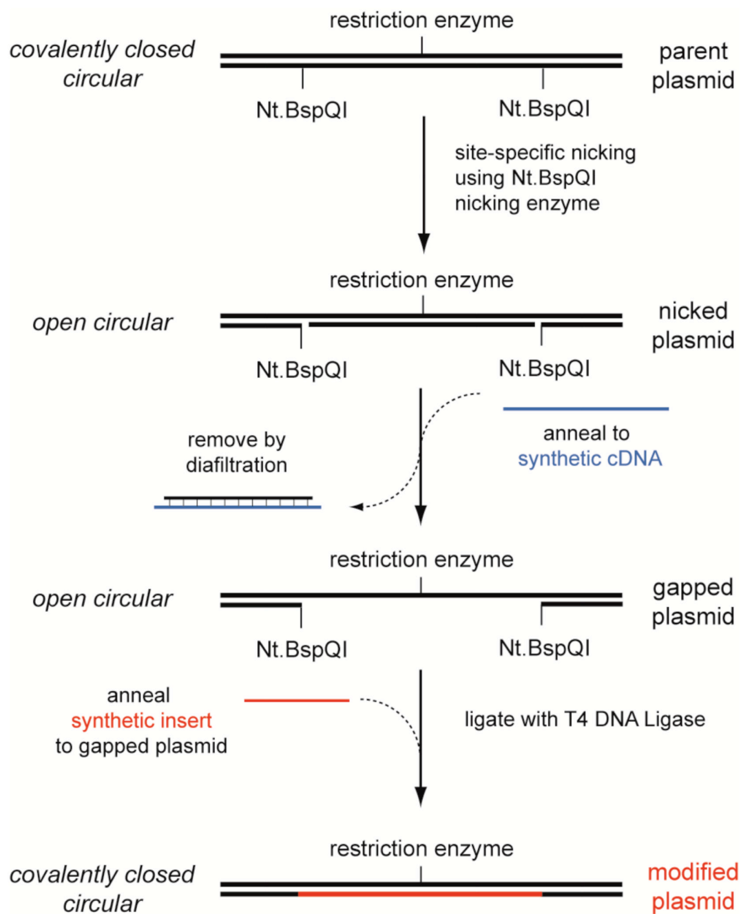
Figure 2. Scheme for preparing site-specifically platinated probes.
