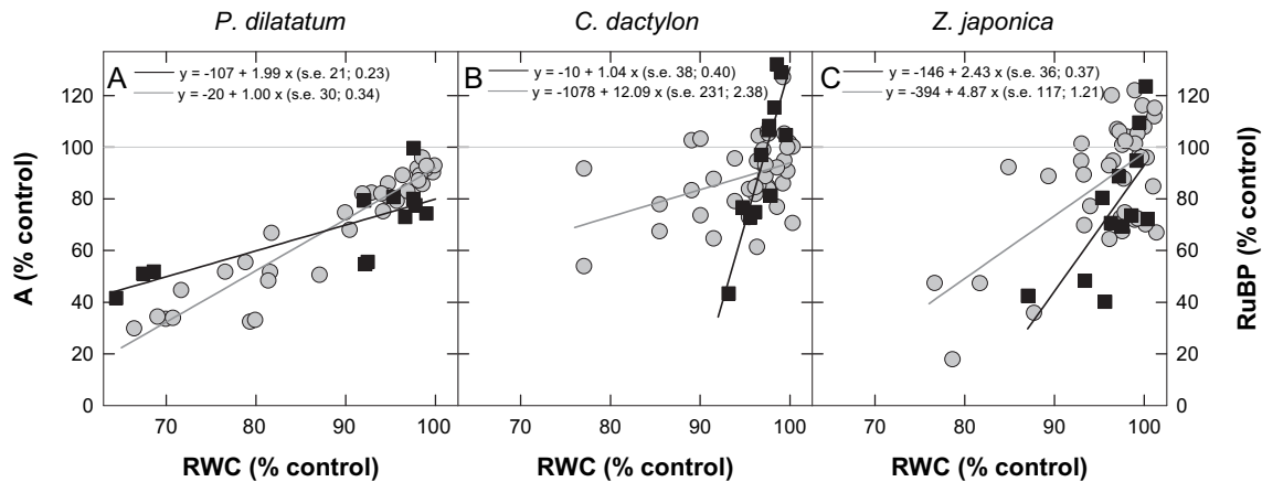
Fig. 3. Effect of leaf dehydration on the quantity of RuBP (black squares) and net \text{CO}_2 assimilation rate ( A , grey circles) of Paspalum dilatatum , Cynodon dactylon , and Zoysia japonica . The RuBP quantities ( \mu\text{mol m}^{-2} ) and rates of photosynthesis ( \mu\text{mol m}^{-2} \text{s}^{-1} ; measured at 25 \pm 2^\circ \text{C} , a PPFD of 850 \pm 50 \mu\text{mol m}^{-2} \text{s}^{-1} , and ambient concentrations of \text{CO}_2 and \text{O}_2 ; Carmo-Silva et al., 2008) obtained for non-watered plants were expressed as a percentage of average values for corresponding control (well-watered) plants, to allow a comparison of drought effects in two independent batches of plants of the three species grown under identical conditions. The relative values of RuBP and photosynthesis were plotted against the corresponding RWC of each drought-stressed sample (also expressed as a percentage of average control values). Each data point corresponds to one sample. Regression lines were fitted when the RWC effect was significant ( F -tests; RuBP: R^2=65.5\% , s^2=220.4 , df=30 ; P < 0.001 ; A : R^2=59.2\% , s^2=198.6 , df=105 ; P < 0.001 ).
