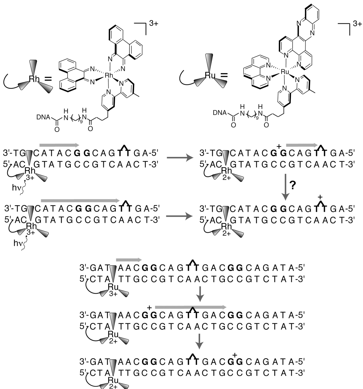
Figure 6. Oxidation and repair of thymine dimer (~1.8 eV) by tethered photoexcited [Rh(φ) 2 (bpy')] 3+ (2.0 V) is unaffected by the intervening double guanine site (1.2 eV). Oxidation of double guanine sites by [Ru(phen)(bpy')(dppz)] 3+ (1.5 eV) is unaffected by the presence of thymine dimer, which this oxidant lacks sufficient driving force to repair. The latter result implies that guanine radical is not competent to repair thymine dimers, in accordance with the known potentials. Hence either the guanine radical oxidized by [Rh(φ) 2 (bpy')] 3+ does not relax prior to migration to the thymine dimer, or the guanine radical is not an intermediate in DNA-mediated oxidation of thymine dimer by [Rh(φ) 2 (bpy')] 3+ .
