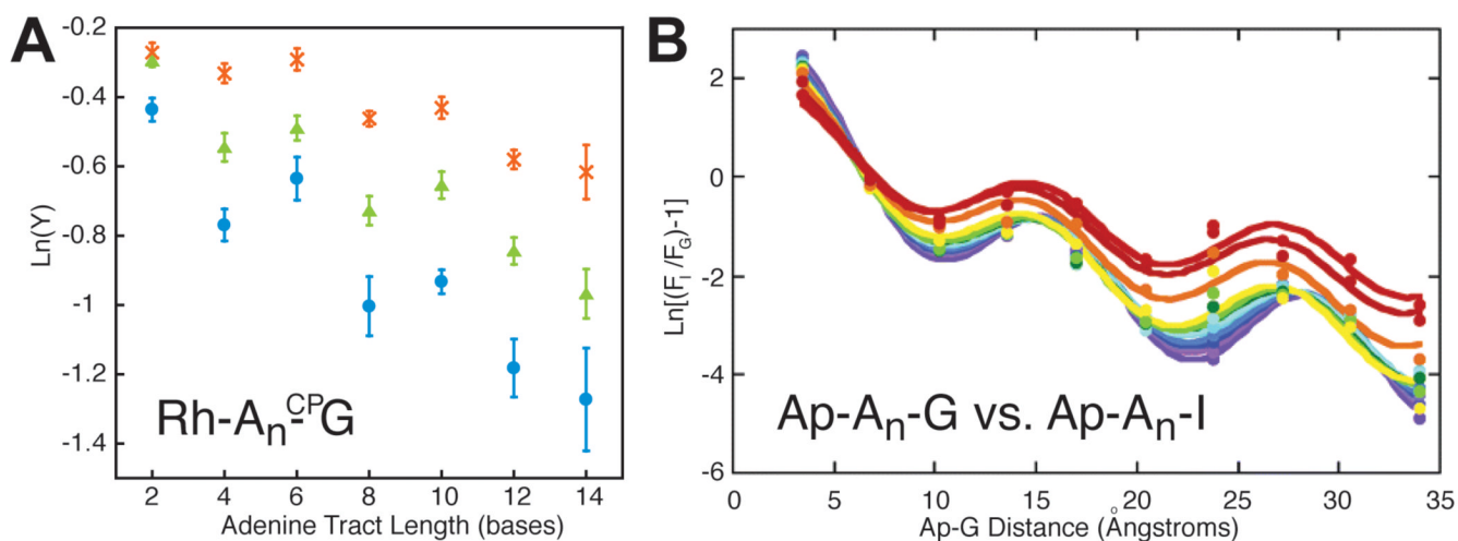
Figure 13. Equivalent periodicities with the same period and temperature dependence are observed for (B) the single-step oxidation of guanine by \text{Ap}^* and (A) the total oxidation of \text{CpG} by photoexcited [\text{Rh}(\text{phi})_2(\text{bpy}') ]^{3+} . Temperature increases from purple to red. Errors are given in (A) as 90% SEM. 54,68 Reprinted with permission from References 54 and 68. Copyright American Chemical Society.
