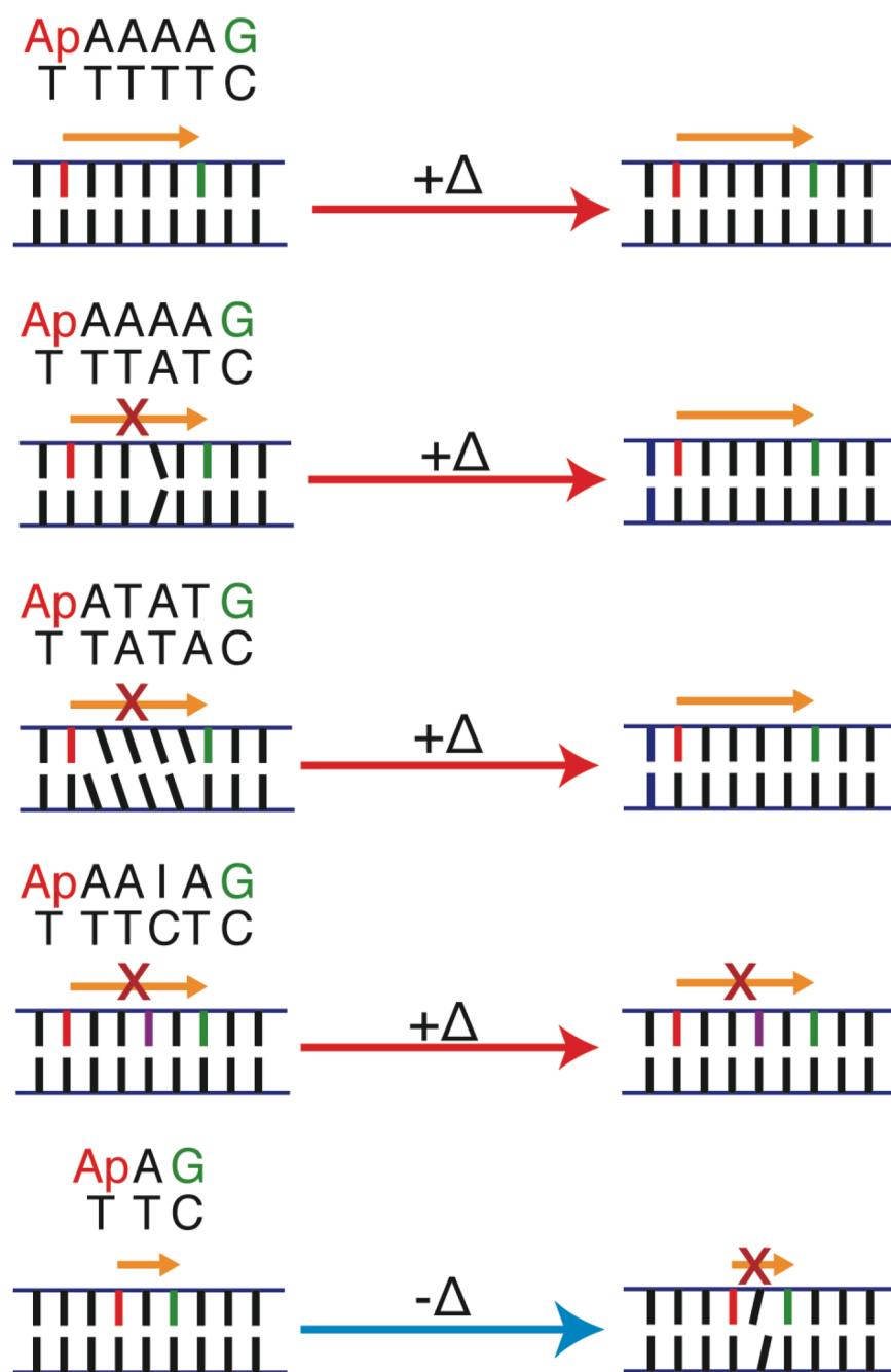
Figure 4. The sequence and temperature dependence of single-step oxidation of guanine by photoexcited 2-aminopurine (Ap) in DNA. 35,54,117 CT yield in well-matched Ap(A) 4 G increases with temperature (+Δ), up to duplex melting. Two perturbations that disturb CT due to poor stacking dynamics, an A–A mismatch and the sequence ATAT, attenuate CT at room temperature but are comparable to the A 4 sequence at higher temperature, while CT through a perturbation that disturbs CT due to an electronic barrier, AAIA, is only partially recovered at high temperature. This argues that the CT activation is related to the flexibility of the bridge. At low temperature (77K), an intervening adenine eliminates CT from Ap to G, implying that the equilibrium conformation is not the CT active conformation.
