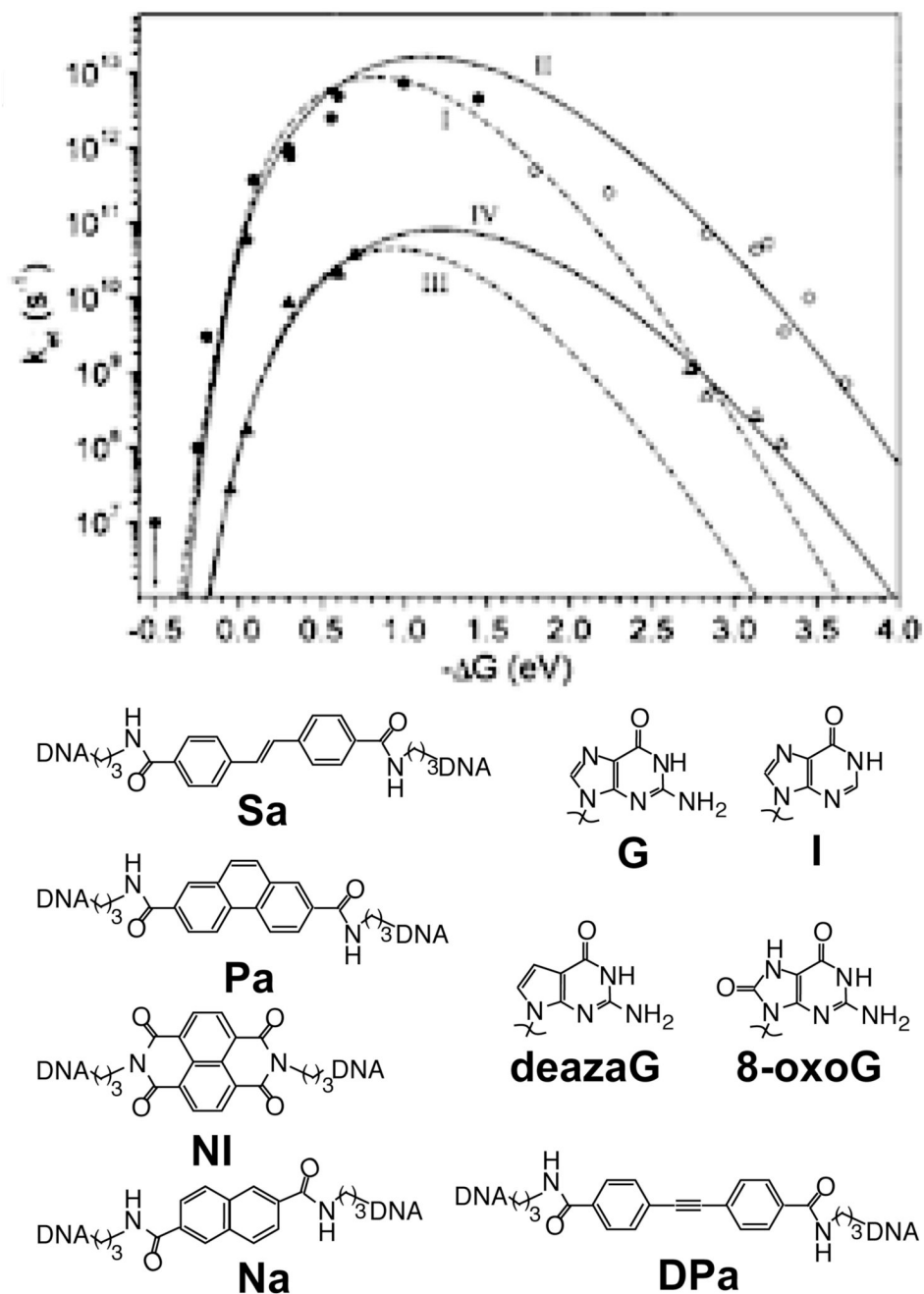
Figure 8. The driving force dependence for CT in photooxidant-bridged DNA hairpins is determined from time-resolved transient absorption studies of a series of five stilbene-derived photooxidants and four hole acceptor bases, following both charge separation (filled) and charge recombination (empty). Case I,II (circles): donor and acceptor are in contact. Case III,IV (triangles): donor and acceptor are separated by two TA base pairs. Case I,III are fit only to charge separation rates (dotted), while Case II,IV are fit to both charge separation and charge recombination rates (solid). Similar reorganization energies, about 1 eV for the nuclear reorganization energy and \sim 0.2 V for the solvent reorganization energy, are found for both
