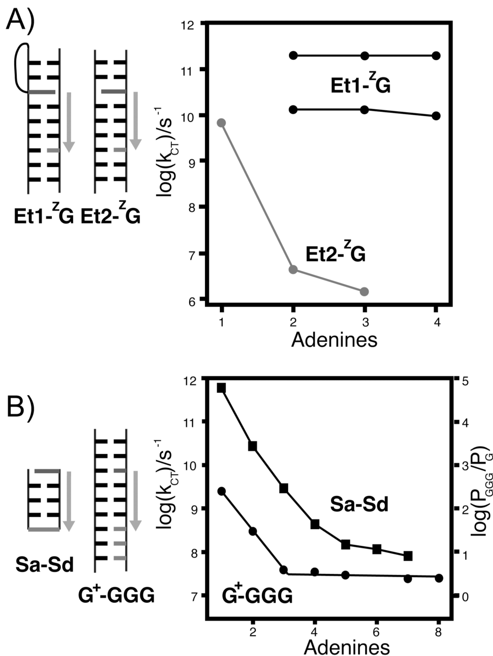
Figure 5. (A) The rate of coherent deazaguanine ( Z G) oxidation by ethidium bromide is the same over short distances for both the flexible linkage ( Et1 , black, both CT rates shown) and the rigid linkage ( Et2 , gray). 27 For two intervening nucleotides, a sharp drop in rate is observed for the rigid Et + , but the rate is unaffected for the flexible Et + . (B) This steep drop in rate over short distances is consistent with that observed for oxidation of guanine by a photoinduced sugar radical (circles), 207 and CT between hairpin capping stilbenes (squares, photooxidation of Sd by Sa ), 125 and has been attributed to a crossover between coherent superexchange and incoherent hopping. In the latter case, comparison of injection and hole arrival rates supports
