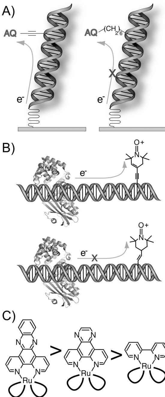
Figure 2. DNA-mediated CT requires electronic coupling to the base pair stack. (A) Electrochemical reduction of an electronically well-coupled anthraquinone (AQ) is facile, while that of a poorly coupled AQ is suppressed. 18 (B) MutY competently reduces an oxidized nitroxide spin label that is well coupled to thymidine, but not the nitroxide conjugated through the partially unsaturated linker. 160 (C) For a series of polypyridyl Ru^{III}(bpy)_2L ground state oxidants, the yield of oxidative damage to DNA scales with the size and planarity of the intercalating ligand. 15
