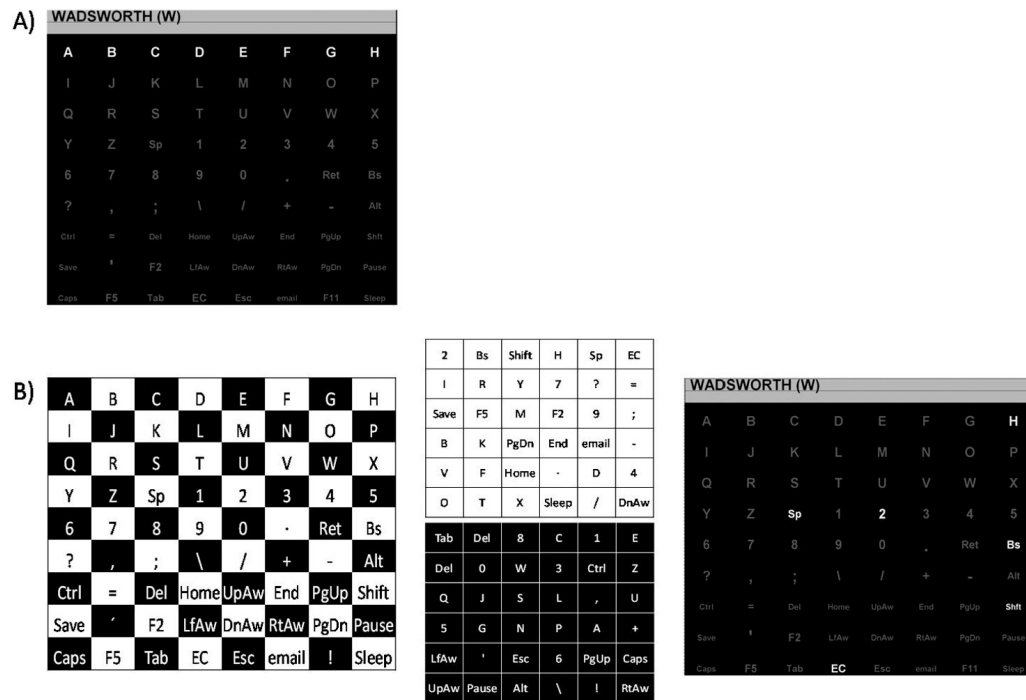
Fig. 1. A: The Row-Column paradigm (RCP) for the 8x9 matrix, with one row flashing. B: The Checkerboard paradigm (RCP) for the 8x9 matrix. On the left is the checkerboard pattern. In the middle are the two virtual 6x6 matrices derived from the checkerboard. On the right is the matrix as presented to the participant with the top row of the white 6x6 virtual matrix flashing. See text for details.
