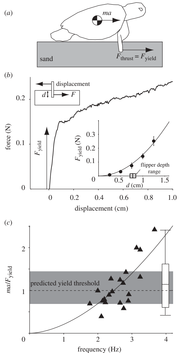
Figure 2. Model of locomotion on sand: (a) flipper ground reaction force F_{thrust} and inertial force ma . (b) Drag force versus displacement shows rapid rise in force (the yield force F_{yield} ) for small initial displacement. Inset: quadratic dependence of F_{yield} on insertion depth d . The bar shows range of measured flipper depths. (c) Normalized turtle inertial force ( ma/F_{yield} ) versus limb frequency (fit curve is ma/F_{yield} = cf^n ; c = 0.21 , n = 1.74 , r^2 = 0.65 ). Dashed line indicates predicted yielding threshold for a single flipper inserted to average measured turtle depth (grey region is yield for mean \pm s.d. depth).
