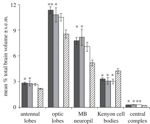
Figure 2. Mean percentage ( \pm s.e. of the mean) of total brain volume for each brain region. Asterisks indicate values significantly different from young, 1-day-old bees (Tukey's HSD pairwise comparisons). One, two and three asterisks indicate p -values < 0.05 , < 0.005 and < 0.0005 , respectively. Black bars, solitary; grey bars, queen; white bars, worker; striped bars, young.
