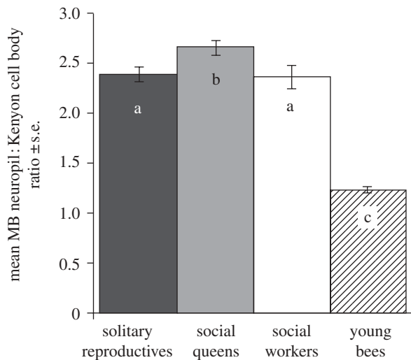
Figure 3. MB neuropil:Kenyon cell body ratio for each group. Bars with different letters are significantly different from each other; see text for statistics.
