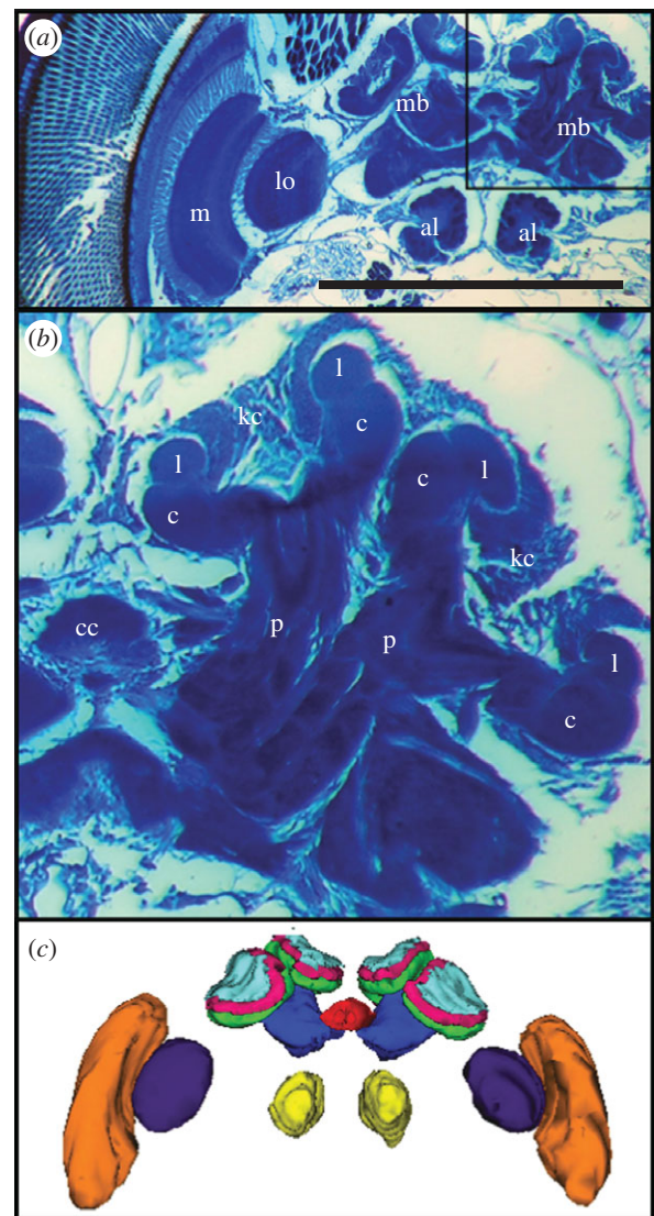
Figure 1. (a) Section of M. genalis brain including the left compound eye, medulla (m), lobulla (lo), both mushroom bodies (mb) and antennal lobes (al). Scale bar, 1 mm. The box in the upper right is enlarged in (b) to show the central complex (cc) and subunits of the mushroom body: peduncle (p), collar (c) lip (l) and Kenyon cell bodies (kc). (c) Three-dimensional reconstruction of the M. genalis brain from serial histological sections. The medulla is orange, lobulla purple, antennal lobe yellow, peduncle royal blue, central complex red, collar green, lip pink and Kenyon cells sky blue.
