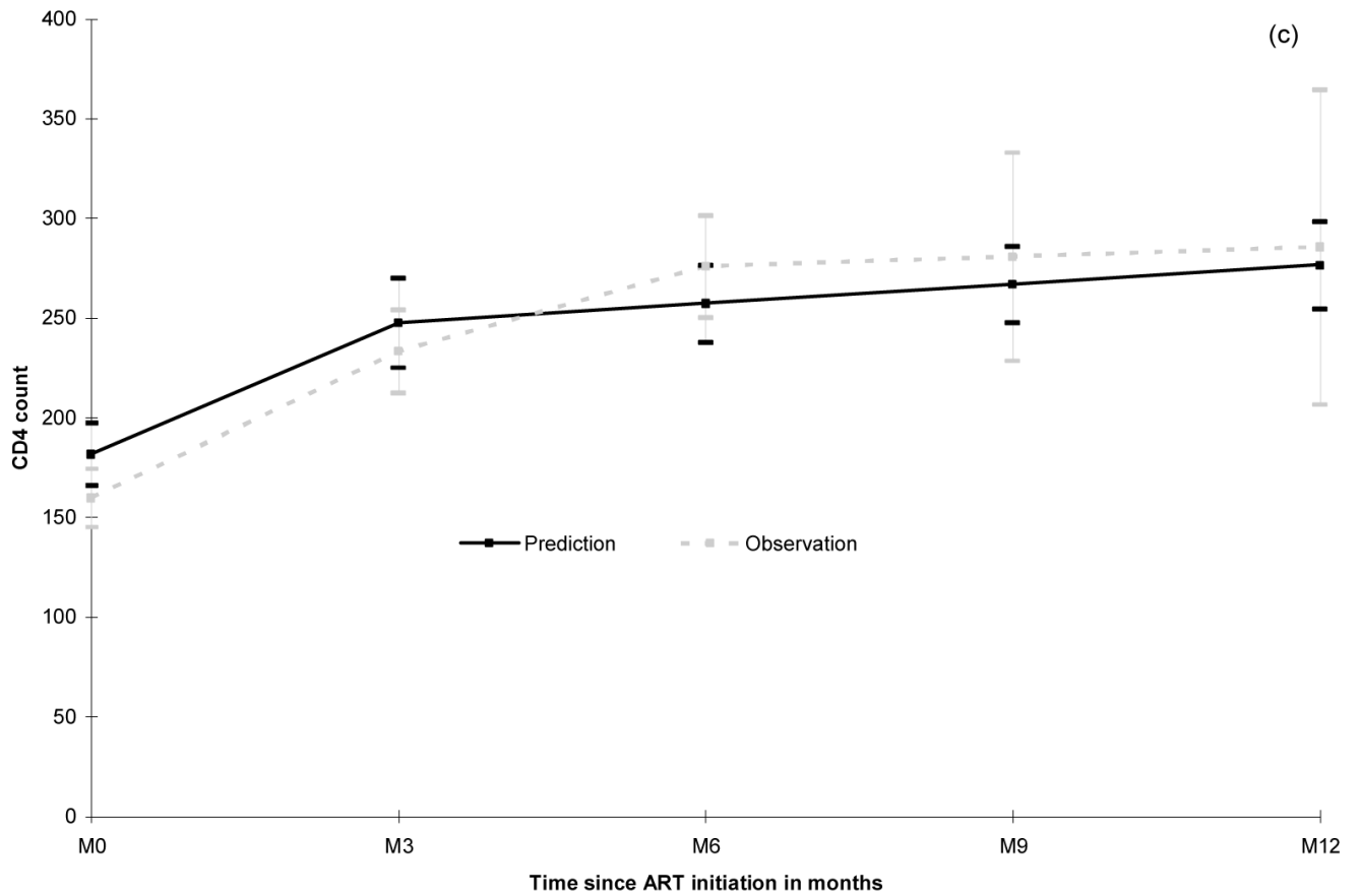
Figure 2. Predicted (from piecewise linear mixed model) and observed mean values of CD4 absolute count (95% Confidence Interval) for HIV-1 (a), HIV-2 (b) and dually positive patients (c). IeDEA West Africa Collaboration.
