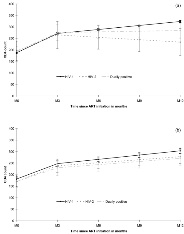
Figure 3. Estimated mean CD4 response (95% Confidence Interval) during the first year of treatment by HIV type in patients treated with NNRTI (a) and treated with PI (b).
