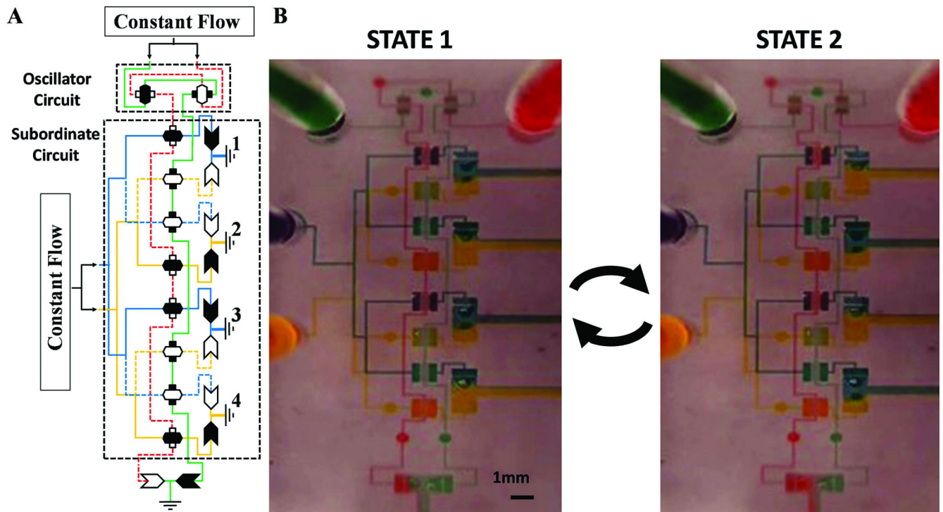
Fig. 3. Fluidic oscillator controls flow in subordinate fluid-circuit
