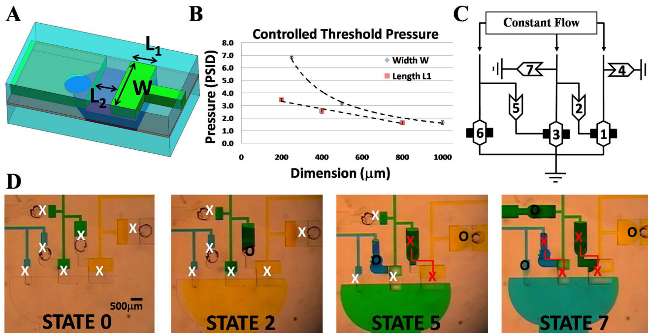
Fig. 4. Automated Fluid Circuits for Cascading Operations
