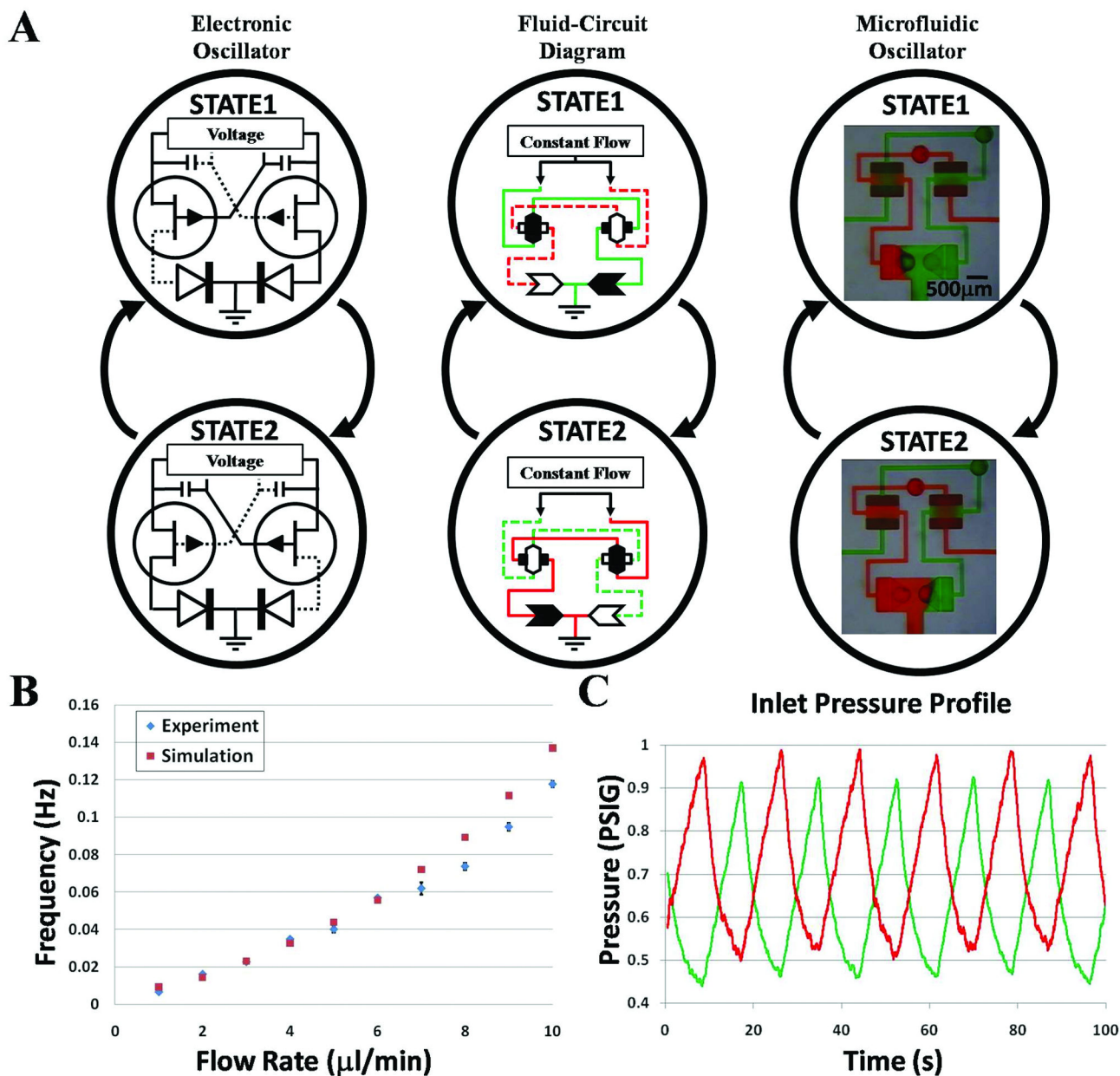
Fig. 2. Interactive elastomeric components for oscillatory switching (A) Comparison between microfluidic oscillator and electronic oscillator. The two states of a microfluidic oscillator automatically produce an alternating output flow between two distinct solutions being simultaneously infused at a constant rate. (B) Graph of both the simulated and experimental data for the oscillators switching frequency for various flow rates within its operating range. Error bars represent the standard deviations from three measurements taken at each flow rate. (C) Graph of pressure oscillations at solution inlets for an infusion rate of 10\mu\text{l}/\text{min} .
