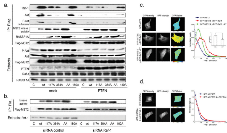
Figure 4. MST2 phosphorylation by Akt at T117 and T384 regulates MST2 kinase activity and Raf-1 interaction
