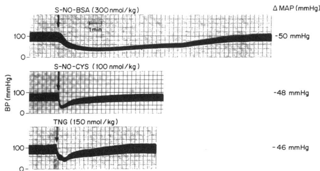
Figure 3. The time course of arterial pressure reduction in response to S -nitroso-BSA, nitroglycerin, and S -nitroso-cysteine. Representative tracings of mean arterial pressure after the intravenous bolus administration of nitroglycerin (TNG), S -nitroso-cysteine (SNO-CYS), and S -nitroso-BSA (SNO-BSA) at equipotent doses.
